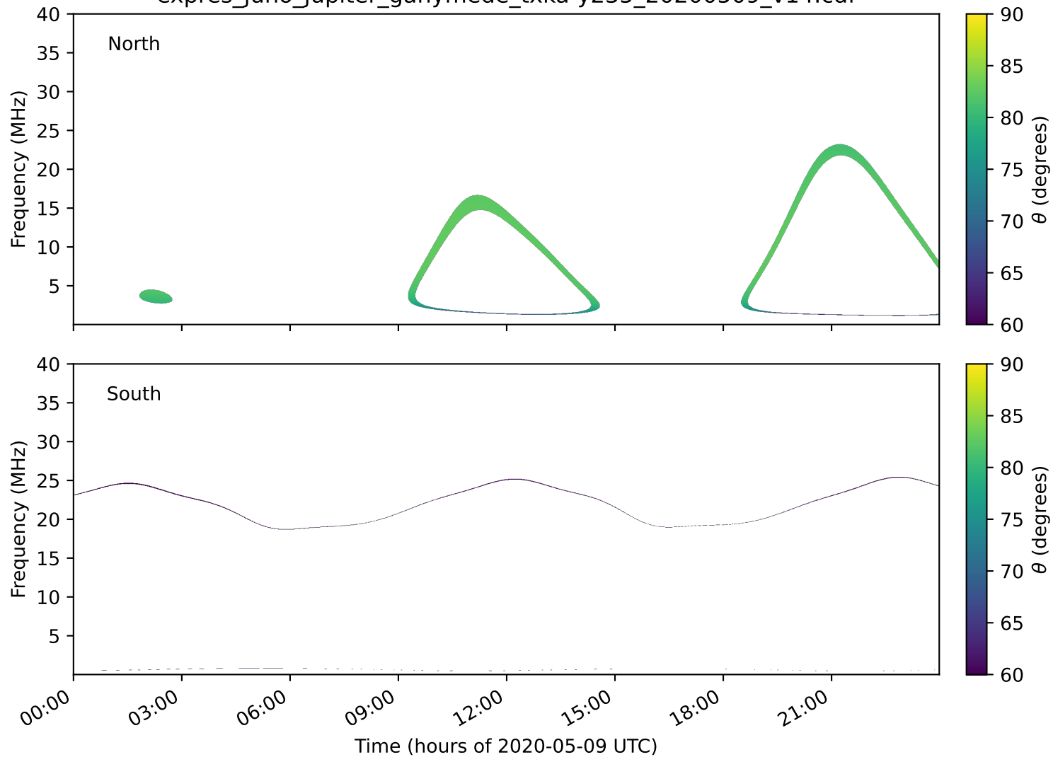
expres_juno_jupiter_ganymede_txka-y235_20200509_v14.cdf
