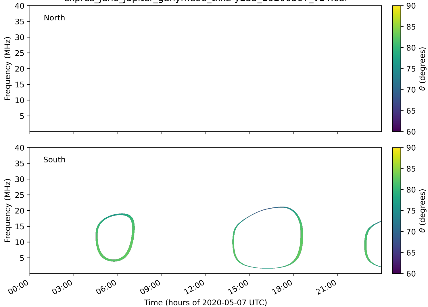
expres_juno_jupiter_ganymede_txka-y235_20200507_v14.cdf
