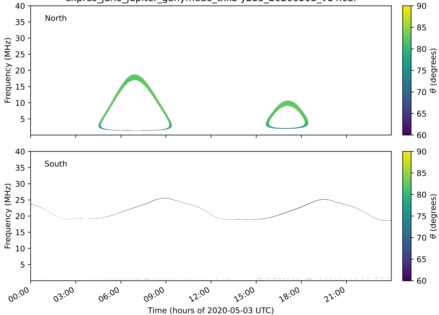
expres_juno_jupiter_ganymede_txka-y235_20200503_v14.cdf
