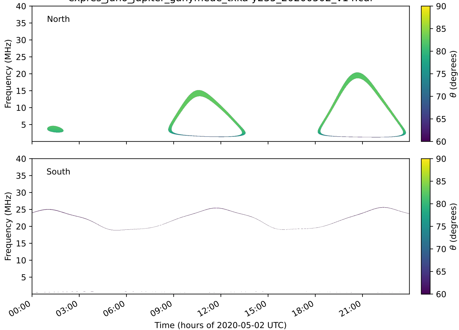
expres_juno_jupiter_ganymede_txka-y235_20200502_v14.cdf
