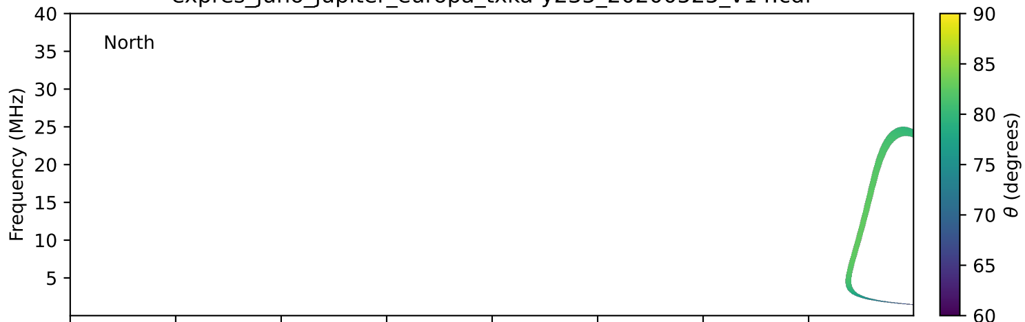
expres_juno_jupiter_europa_txka-y235_20200525_v14.cdf
