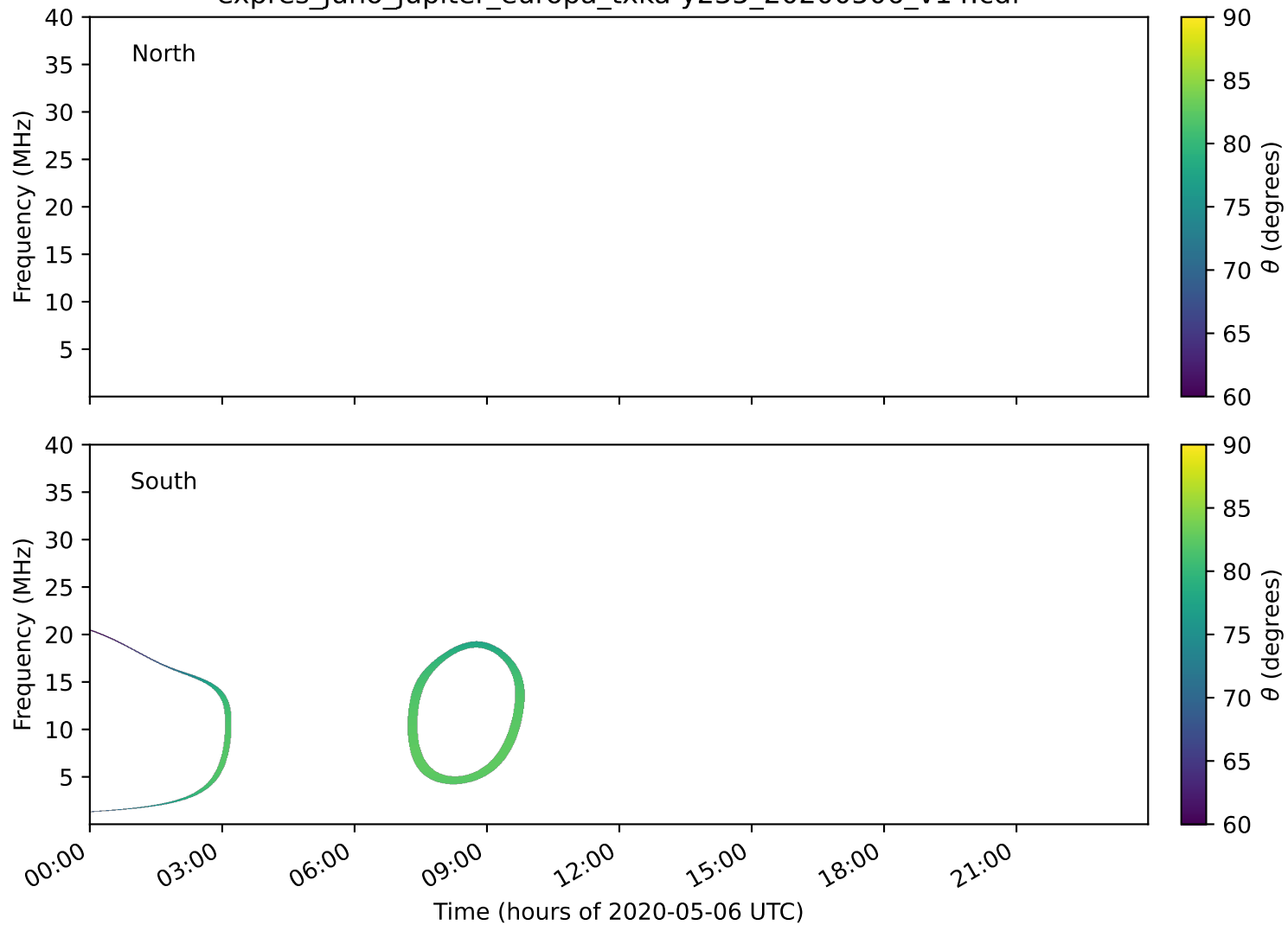
expres_juno_jupiter_europa_txka-y235_20200506_v14.cdf
