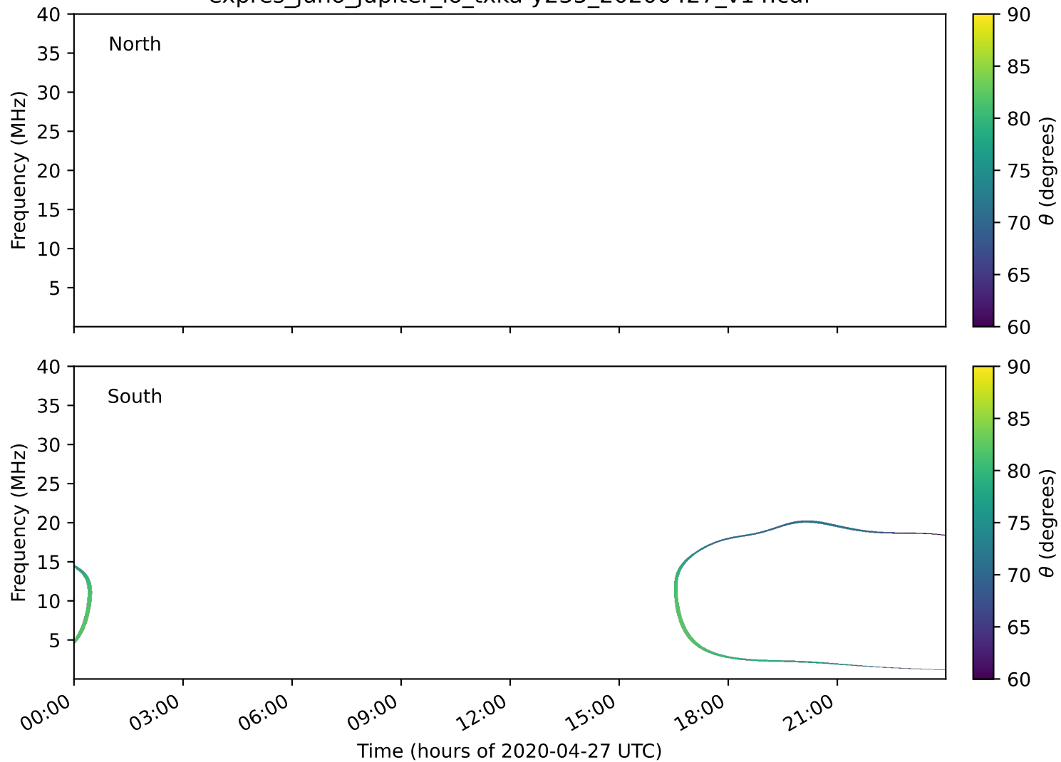
expres_juno_jupiter_io_txka-y235_20200427_v14.cdf
