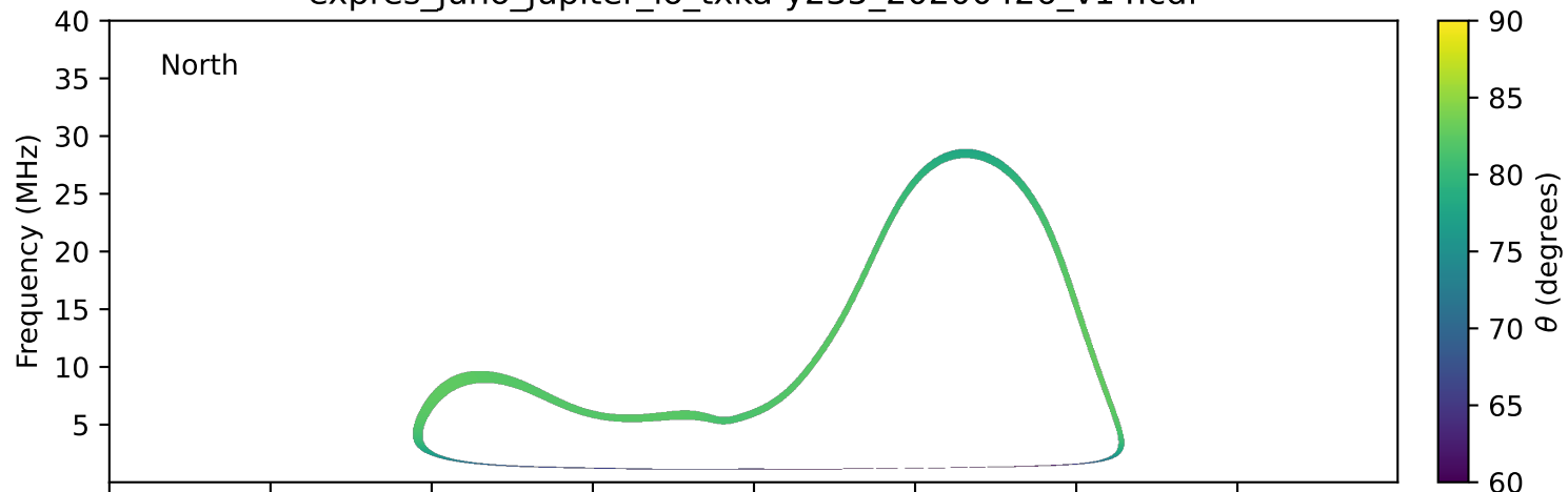
expres_juno_jupiter_io_txka-y235_20200426_v14.cdf
