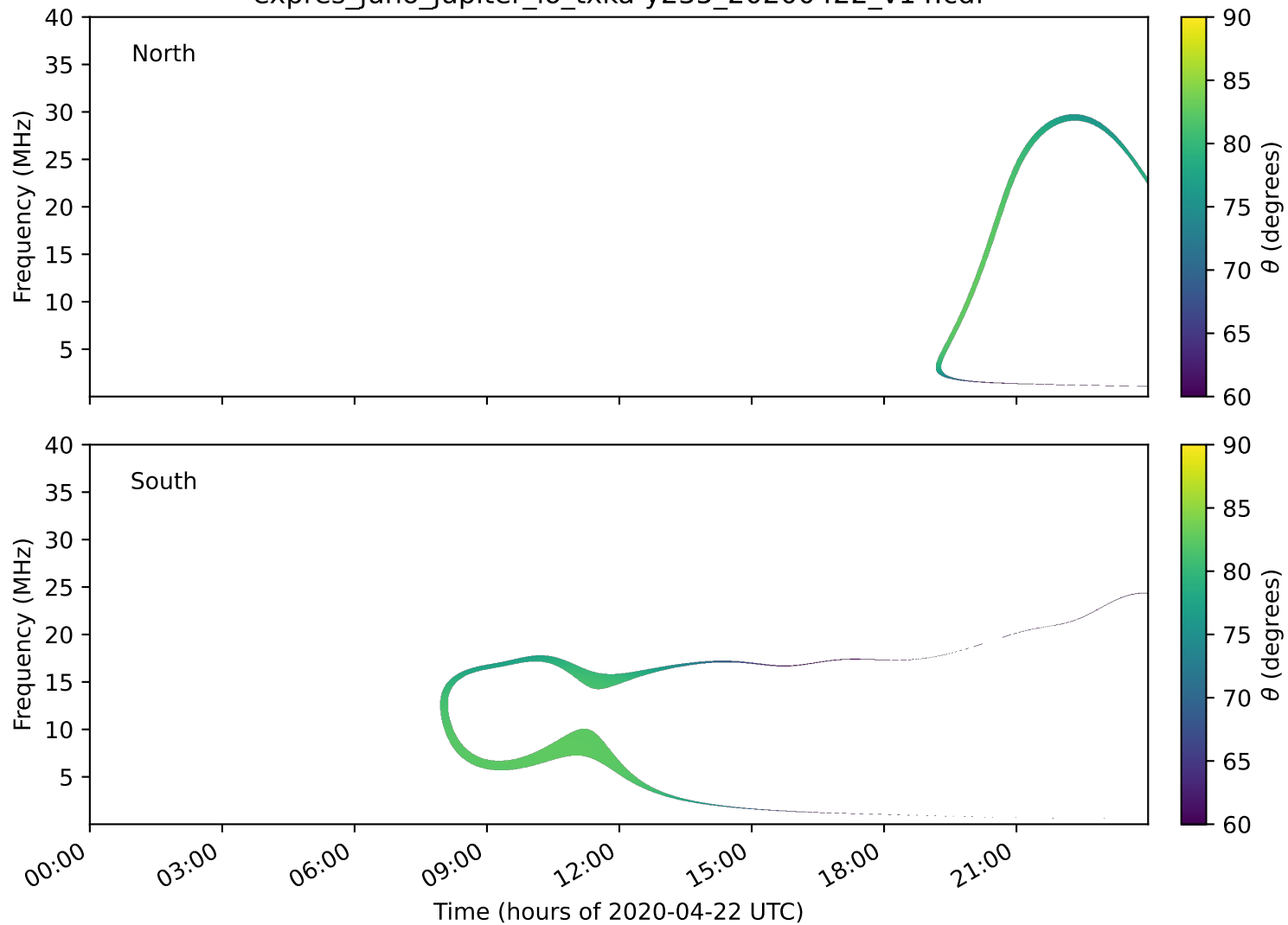
expres_juno_jupiter_io_txka-y235_20200422_v14.cdf
