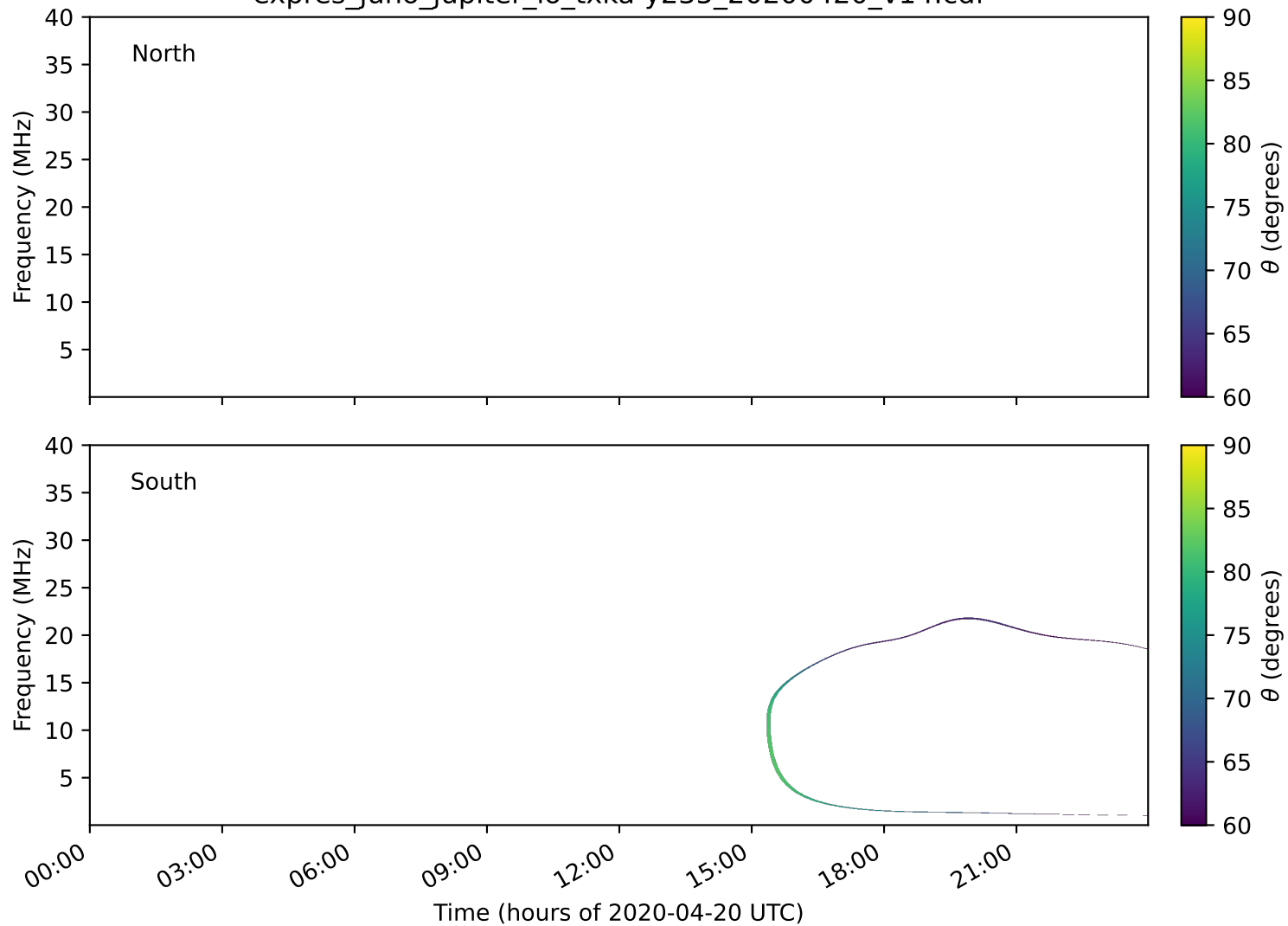
expres_juno_jupiter_io_txka-y235_20200420_v14.cdf
