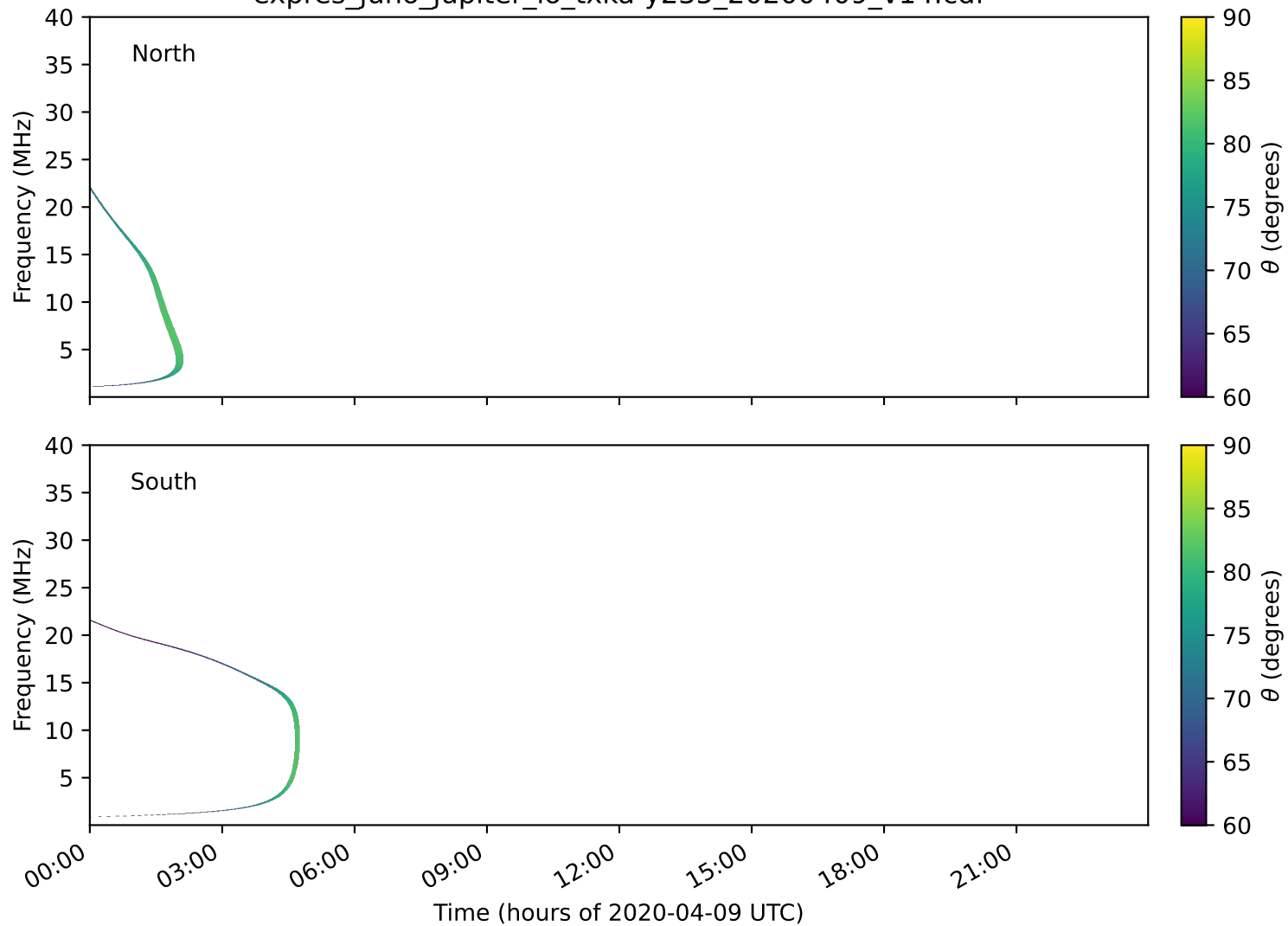
expres_juno_jupiter_io_txka-y235_20200409_v14.cdf
