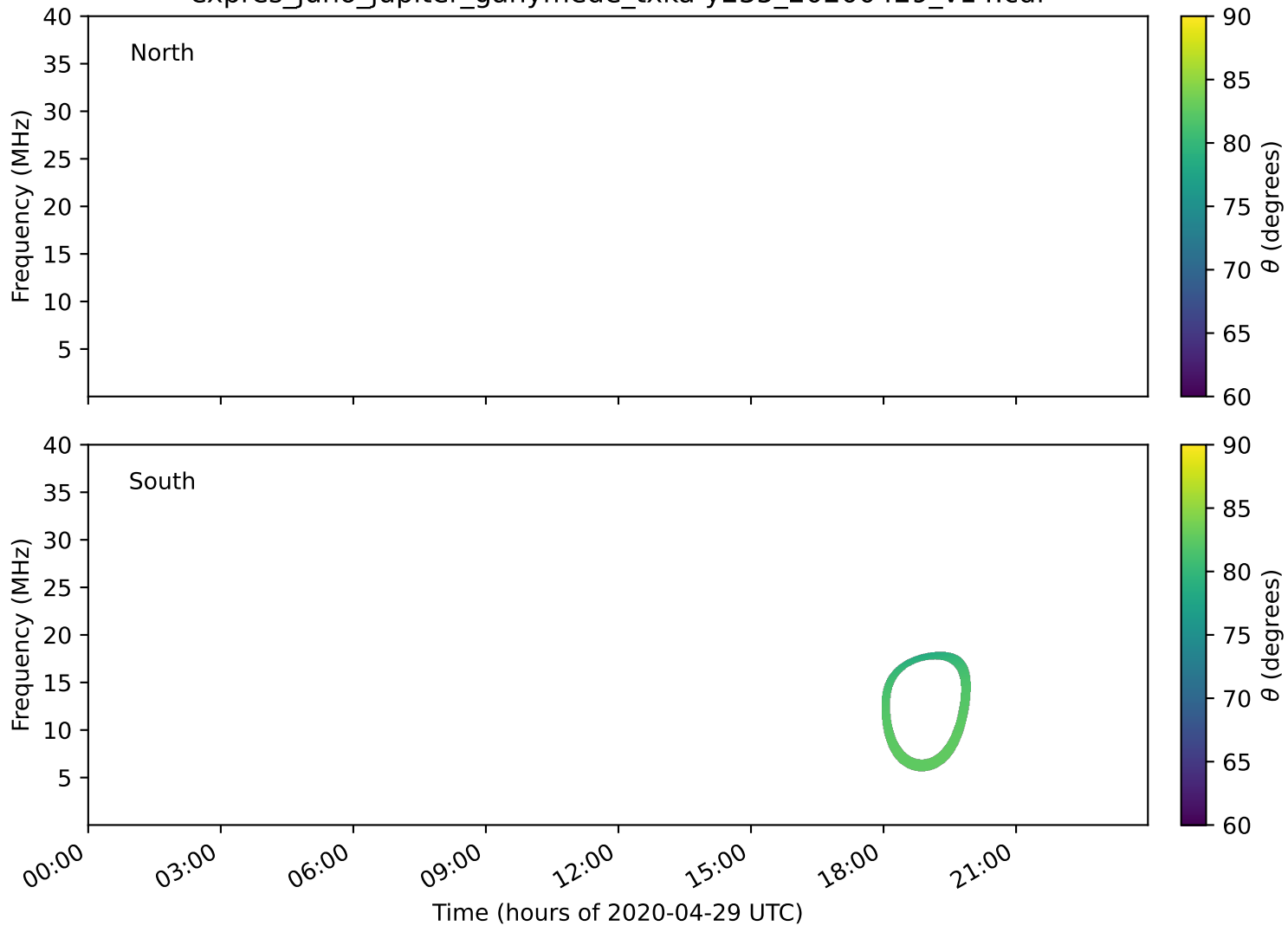
expres_juno_jupiter_ganymede_txka-y235_20200429_v14.cdf
