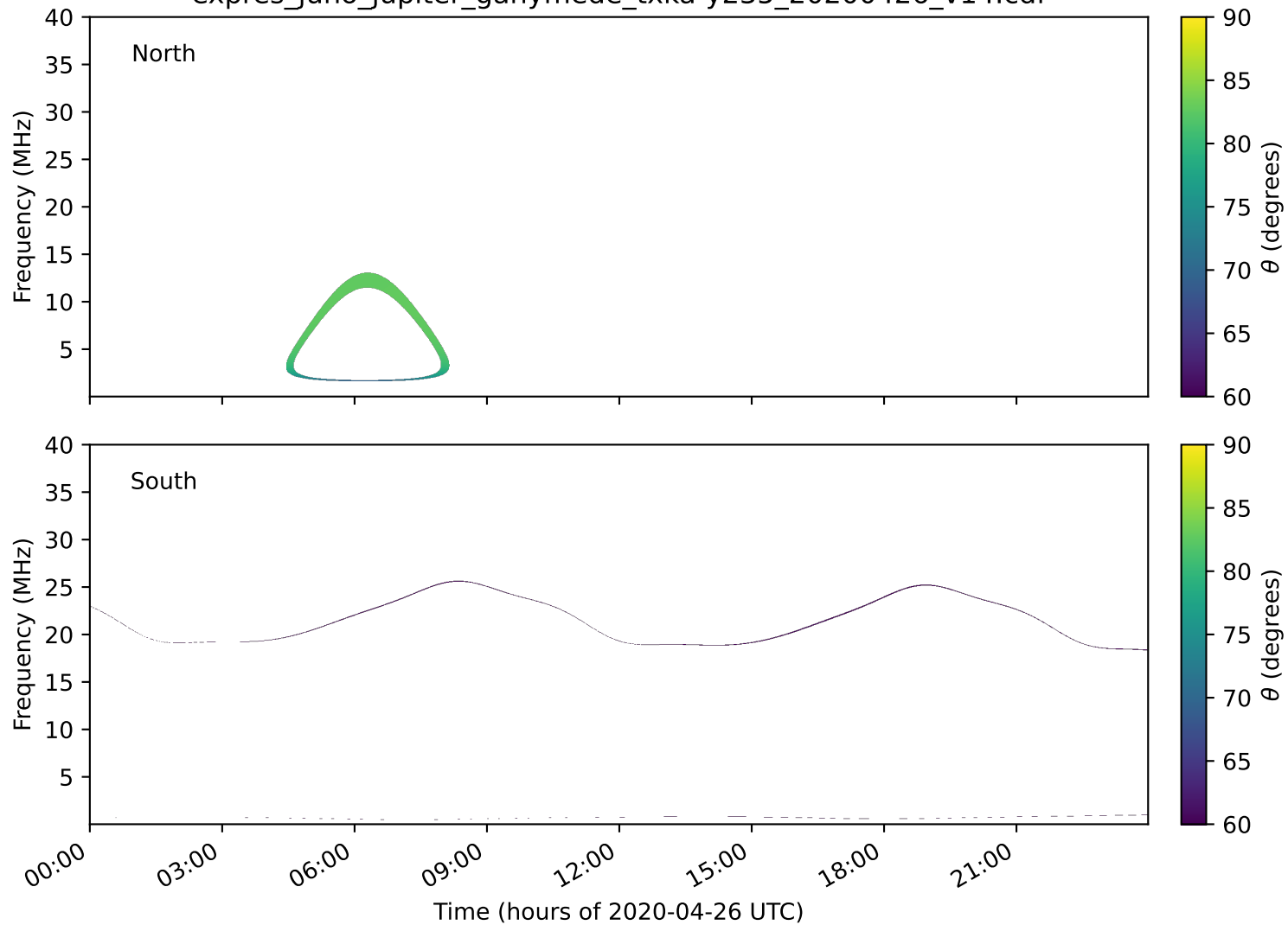
expres_juno_jupiter_ganymede_txka-y235_20200426_v14.cdf
