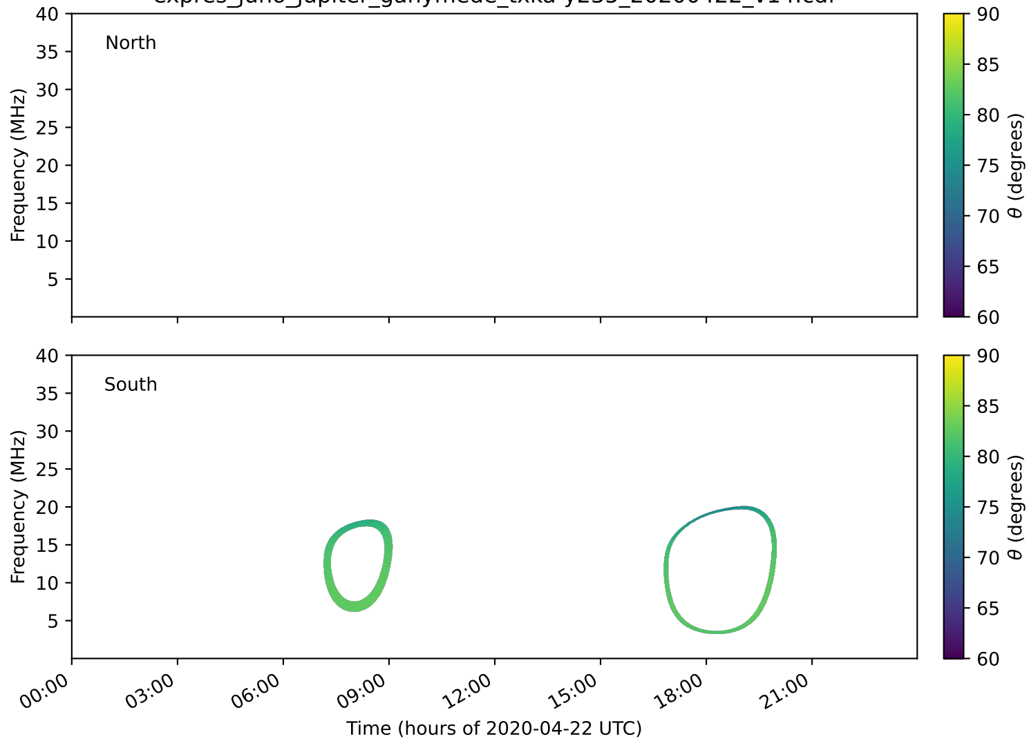
expres_juno_jupiter_ganymede_txka-y235_20200422_v14.cdf
