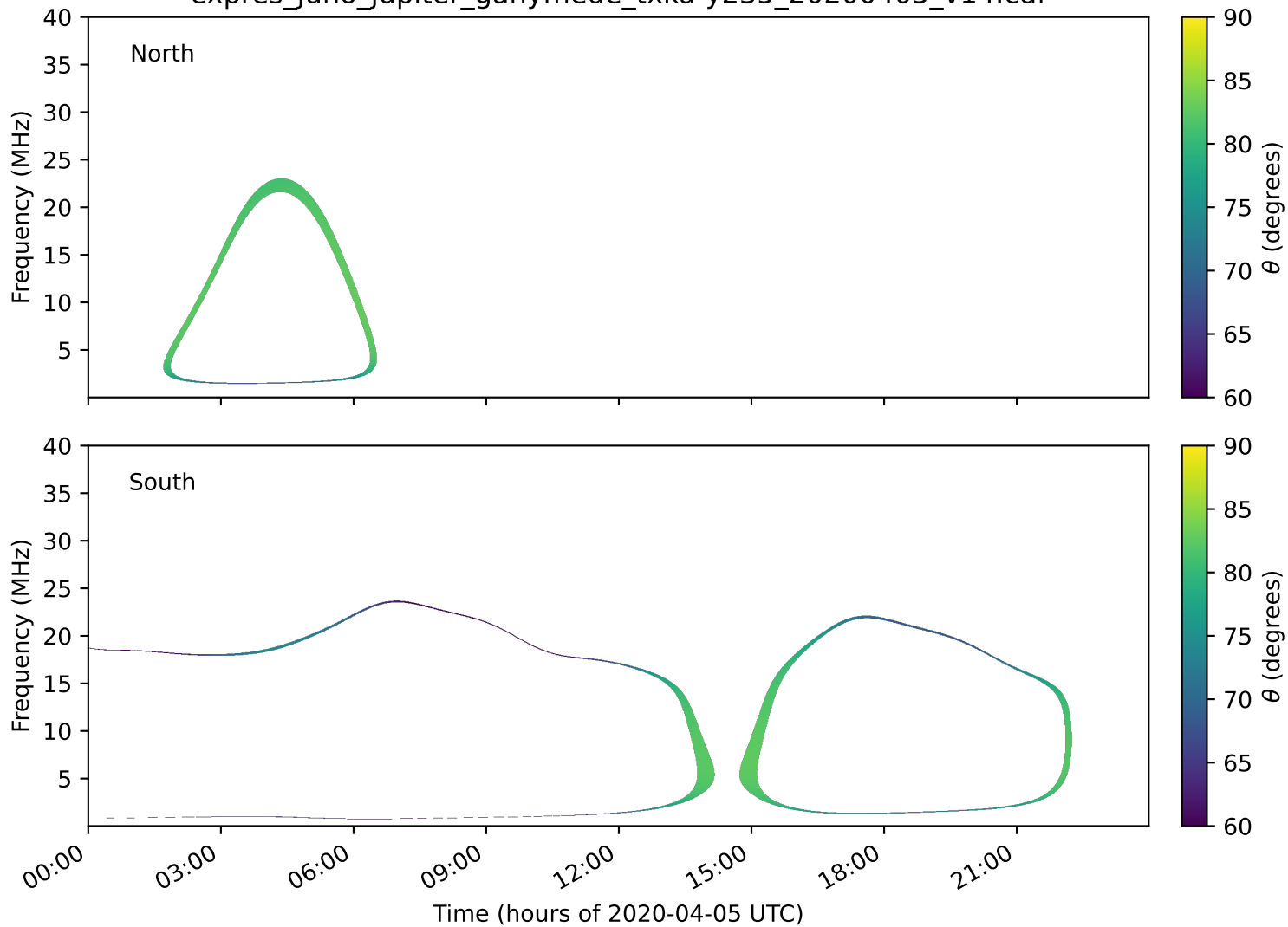
expres_juno_jupiter_ganymede_txka-y235_20200405_v14.cdf
