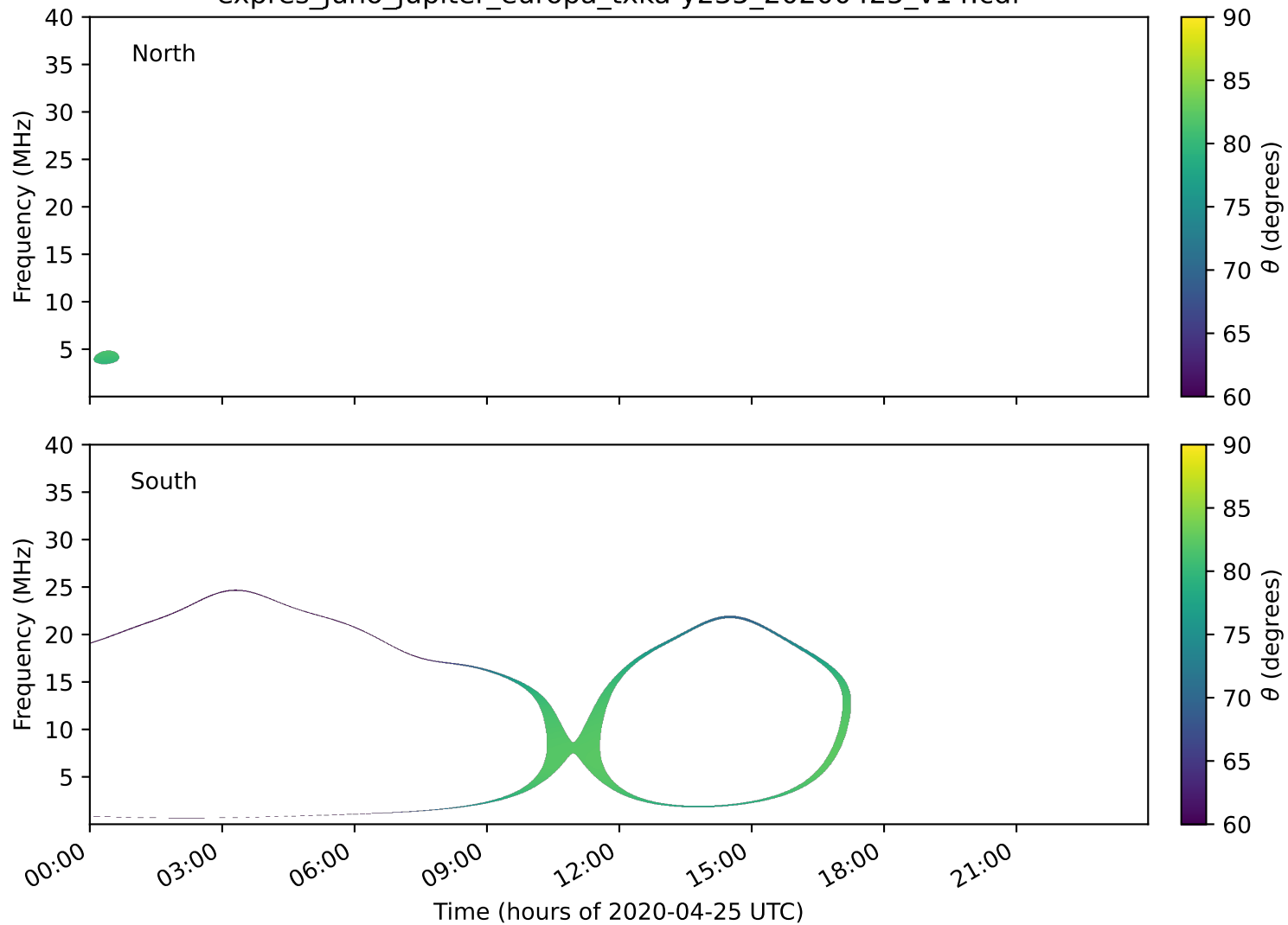
expres_juno_jupiter_europa_txka-y235_20200425_v14.cdf
