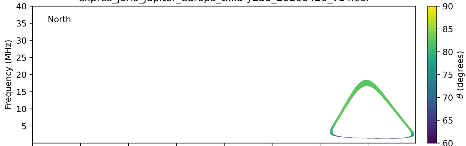
expres_juno_jupiter_europa_txka-y235_20200420_v14.cdf
