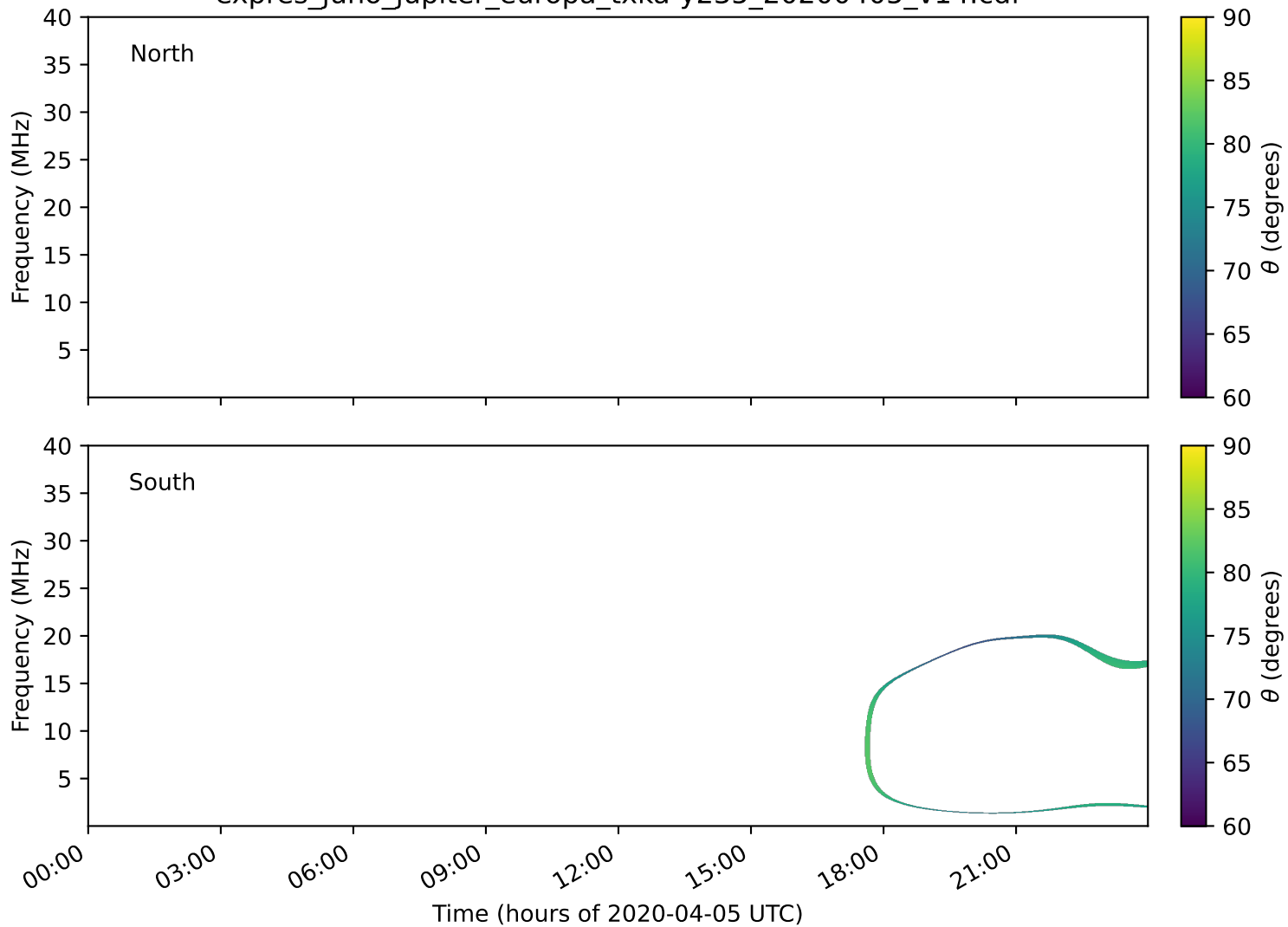
expres_juno_jupiter_europa_txka-y235_20200405_v14.cdf
