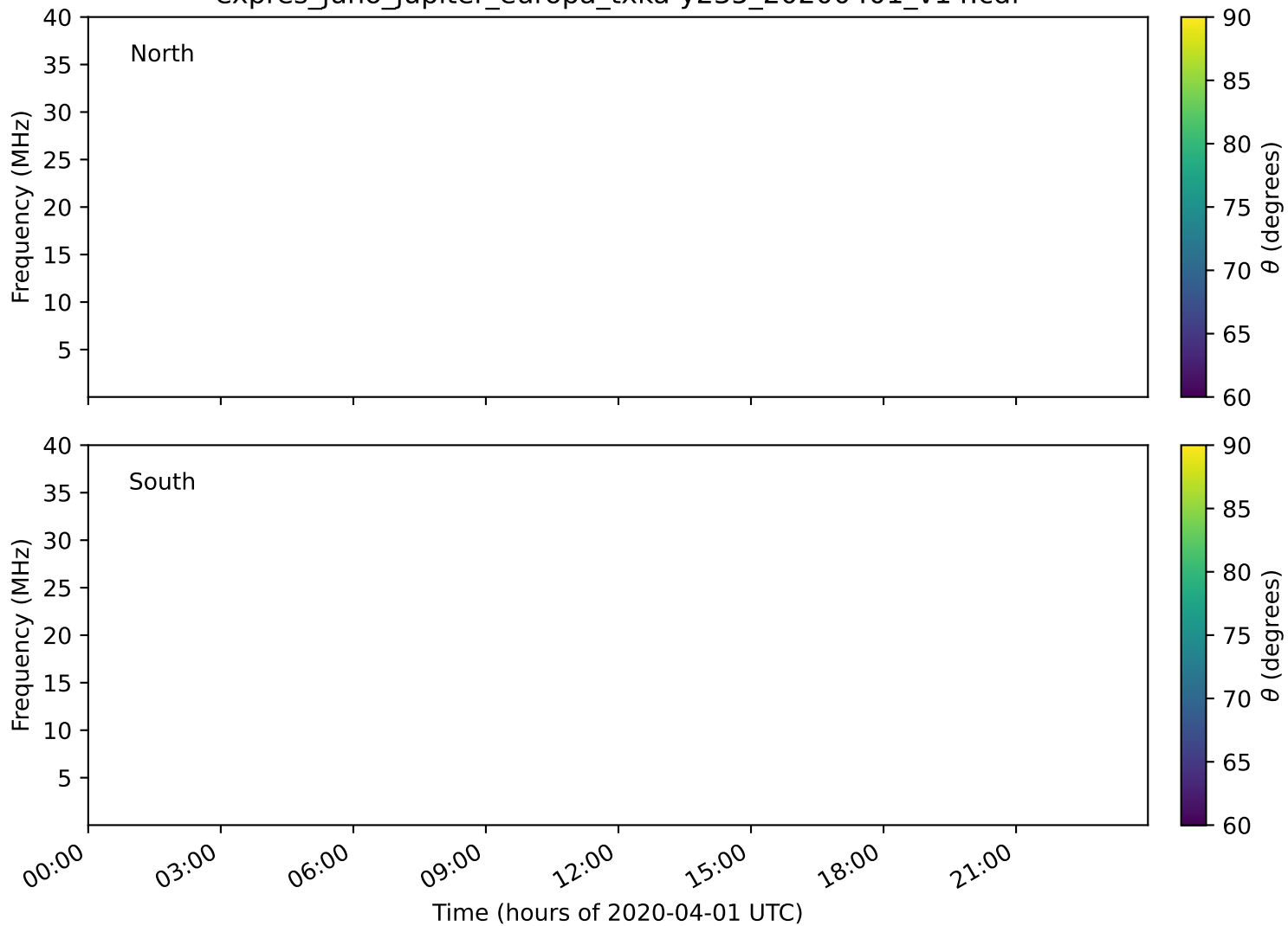
expres_juno_jupiter_europa_txka-y235_20200401_v14.cdf
