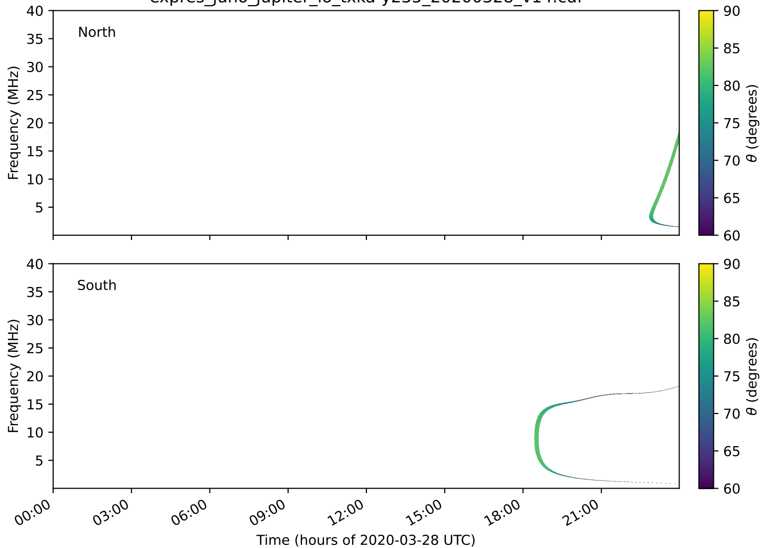
expres_juno_jupiter_io_txka-y235_20200328_v14.cdf
