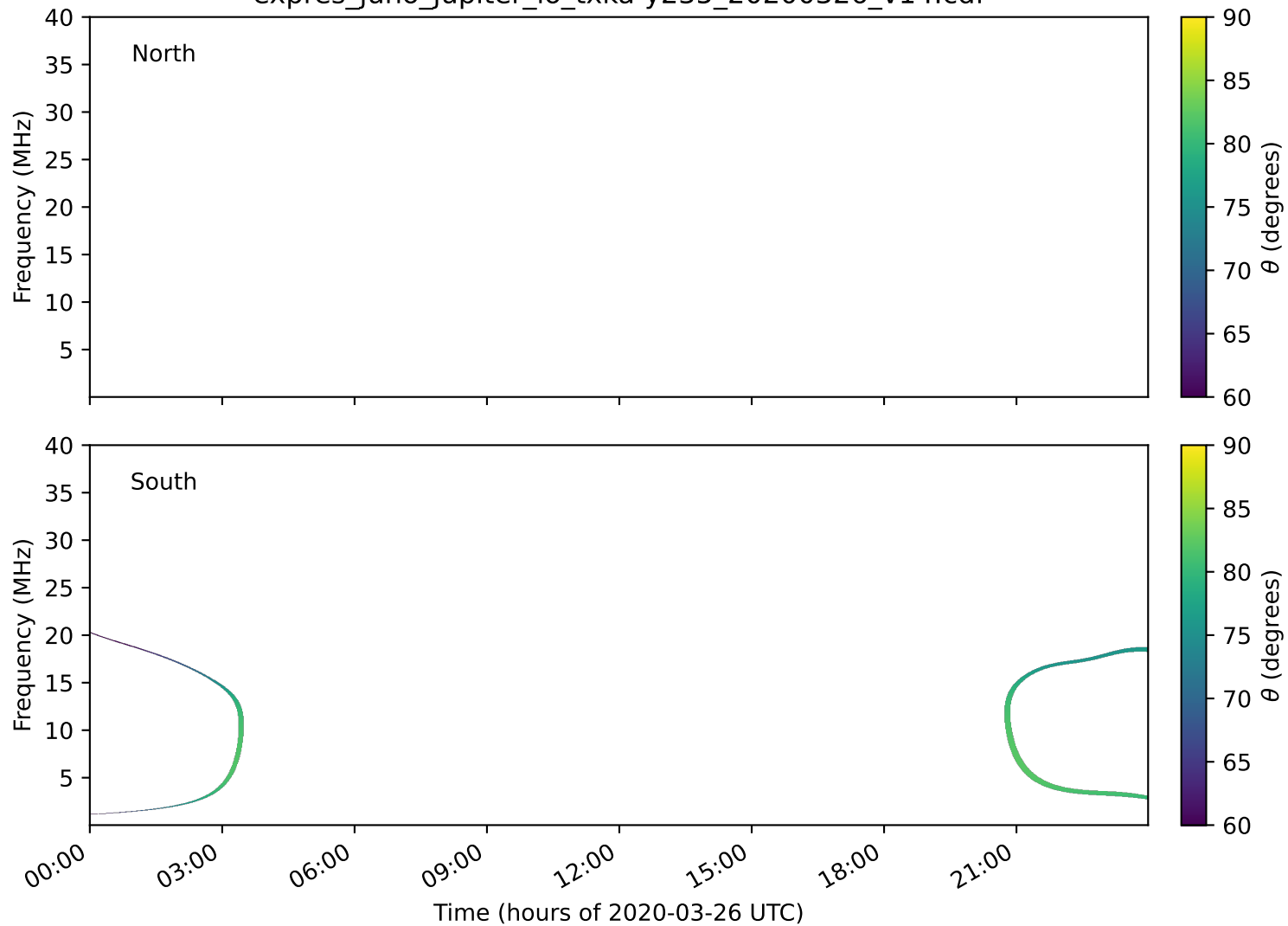
expres_juno_jupiter_io_txka-y235_20200326_v14.cdf
