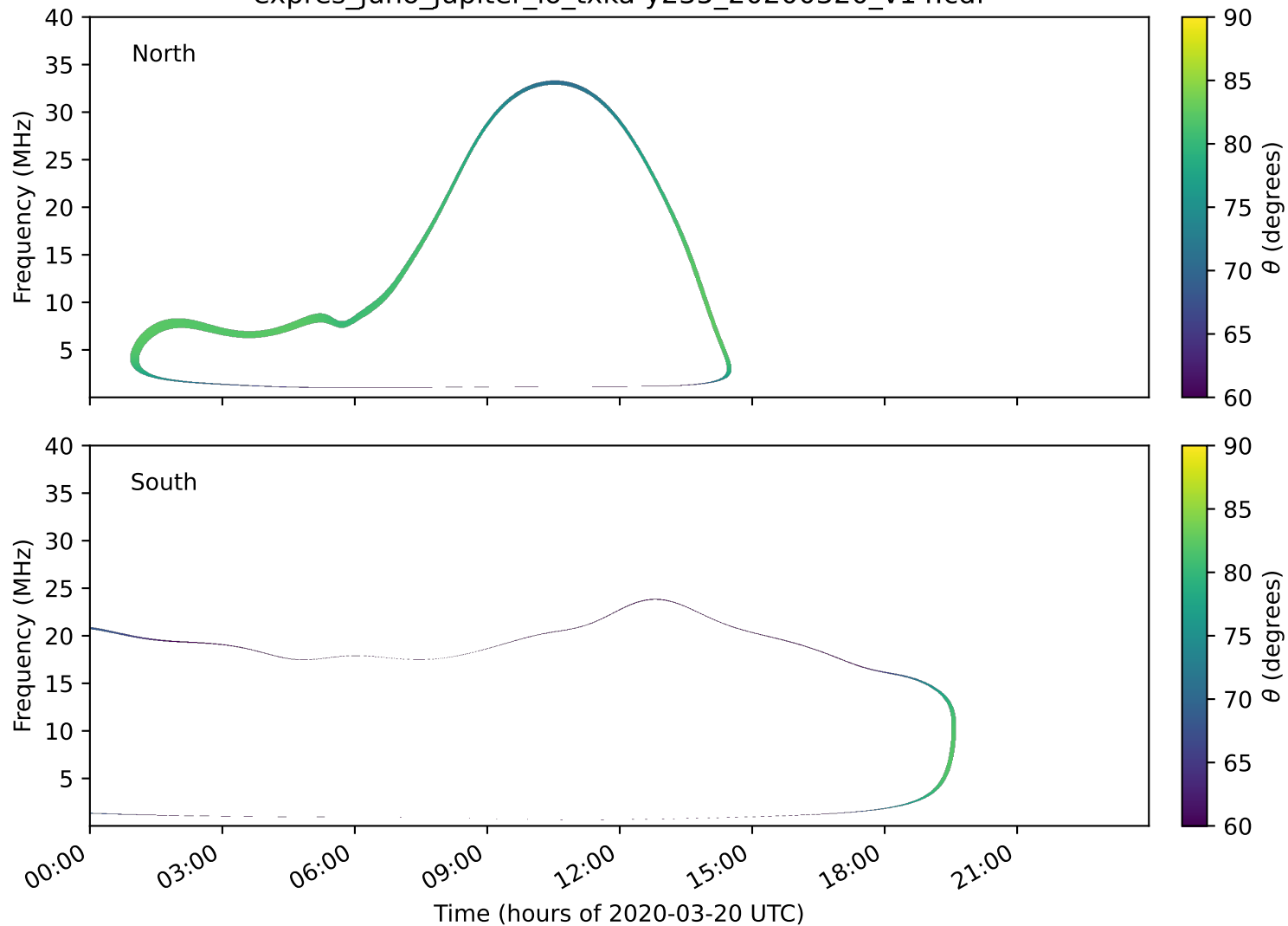
expres_juno_jupiter_io_txka-y235_20200320_v14.cdf
