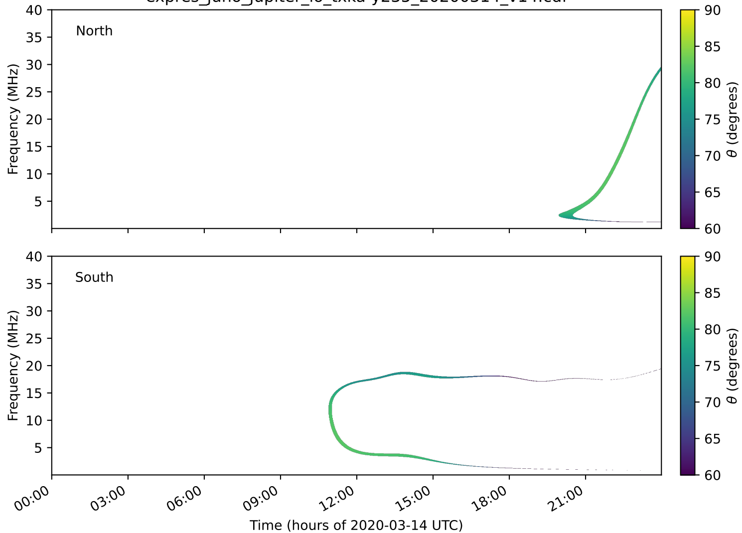
expres_juno_jupiter_io_txka-y235_20200314_v14.cdf
