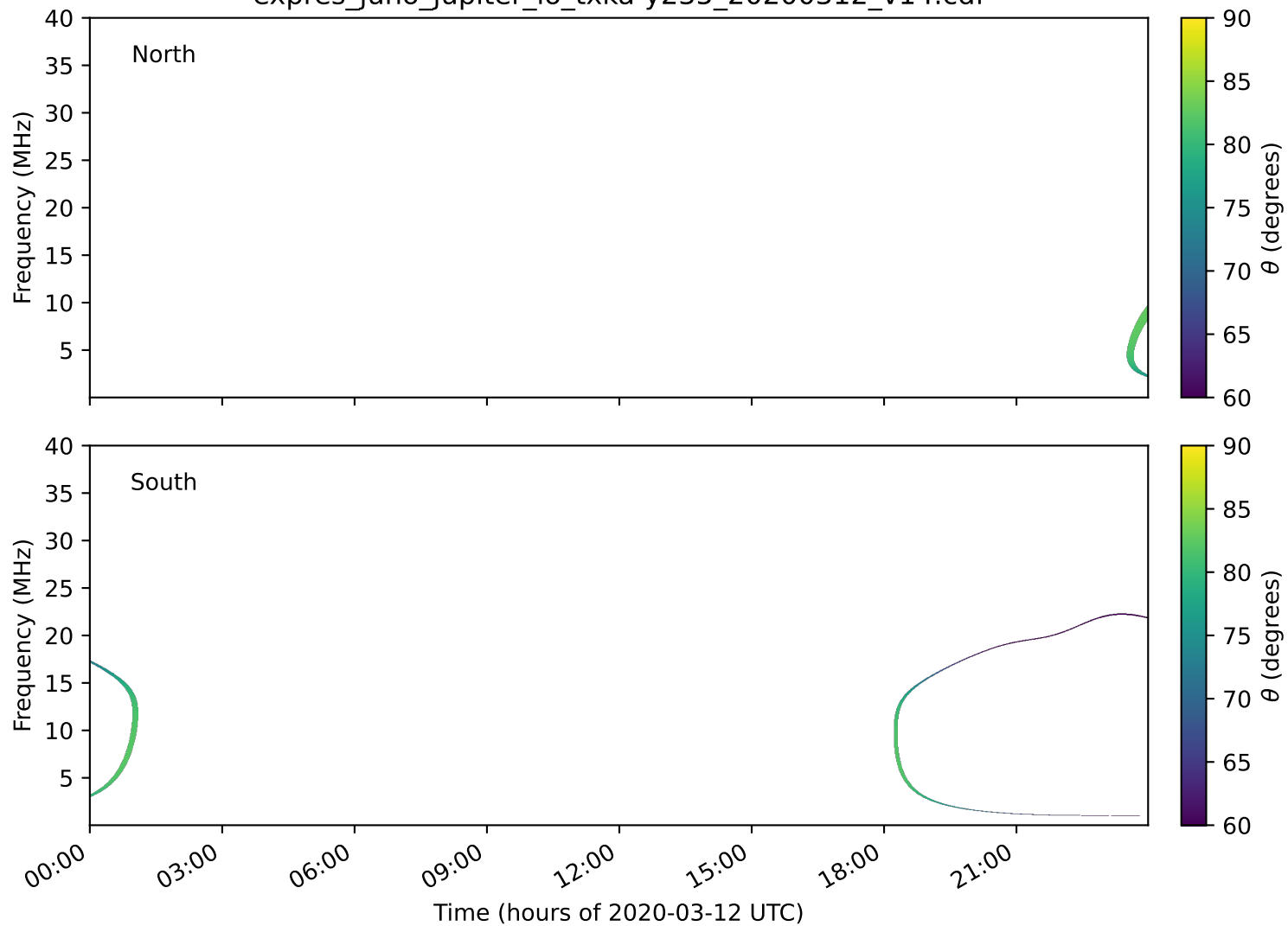
expres_juno_jupiter_io_txka-y235_20200312_v14.cdf
