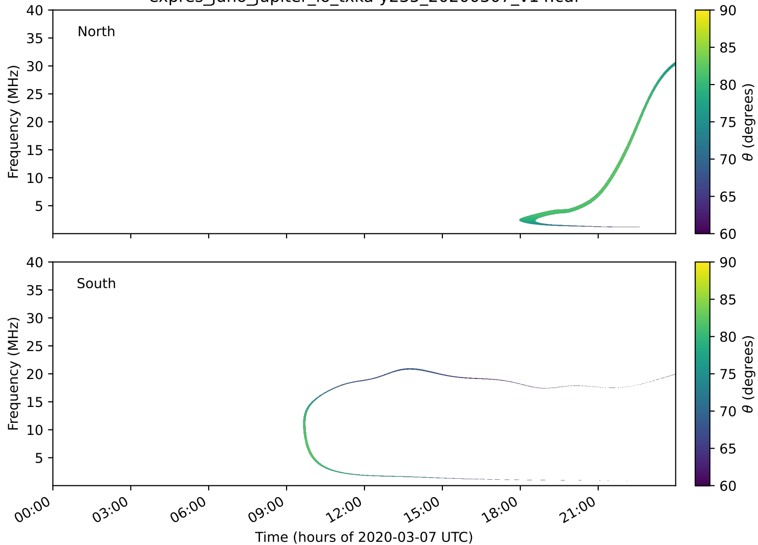
expres_juno_jupiter_io_txka-y235_20200307_v14.cdf
