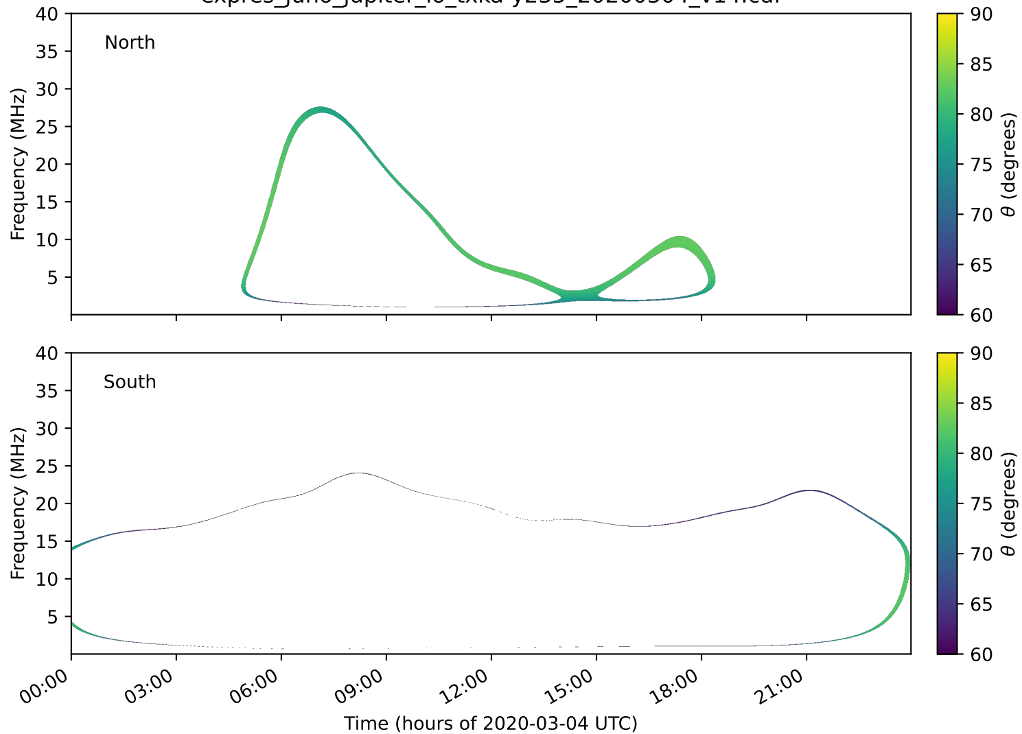
expres_juno_jupiter_io_txka-y235_20200304_v14.cdf
