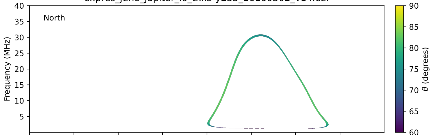
expres_juno_jupiter_io_txka-y235_20200302_v14.cdf
