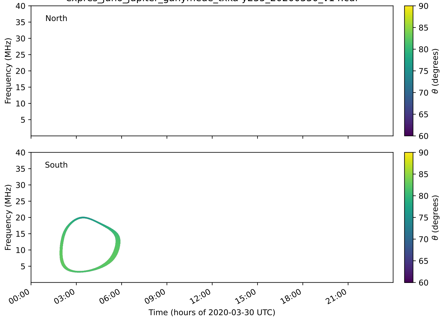
expres_juno_jupiter_ganymede_txka-y235_20200330_v14.cdf
