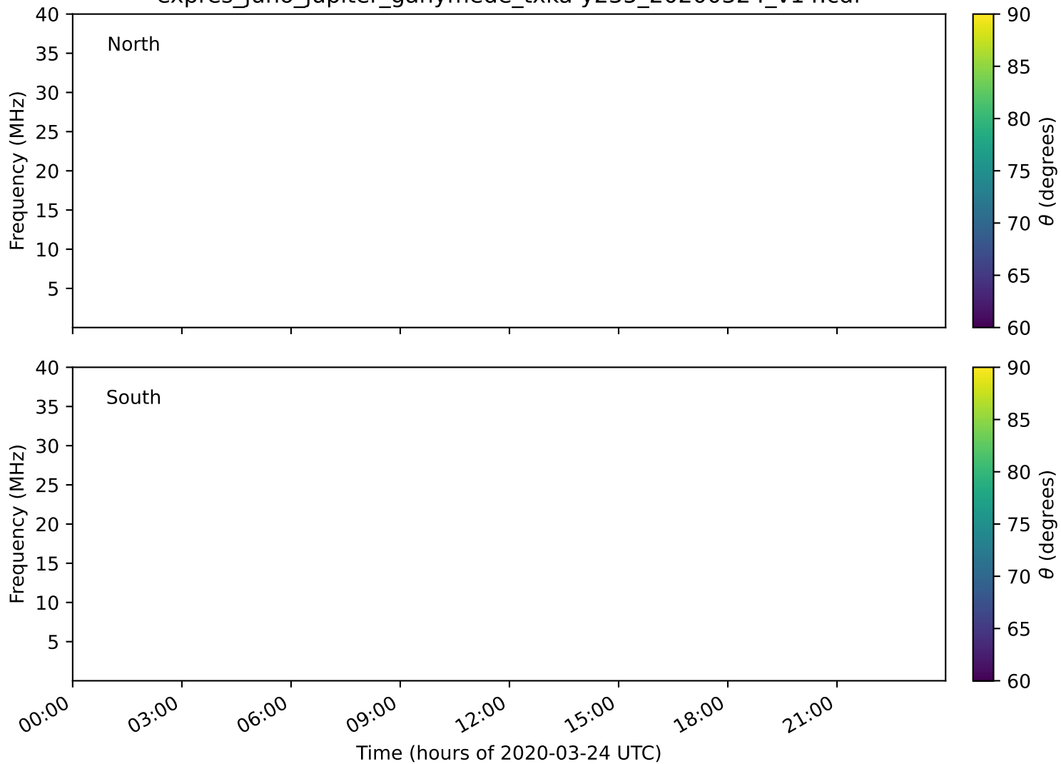
expres_juno_jupiter_ganymede_txka-y235_20200324_v14.cdf
