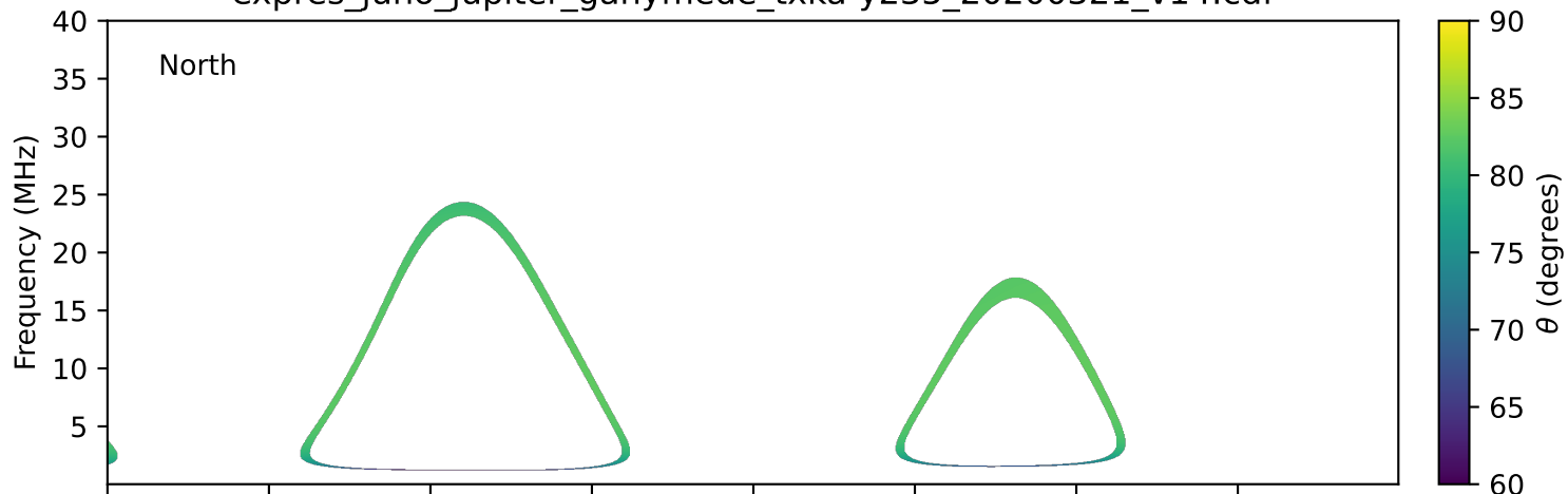
expres_juno_jupiter_ganymede_txka-y235_20200321_v14.cdf
