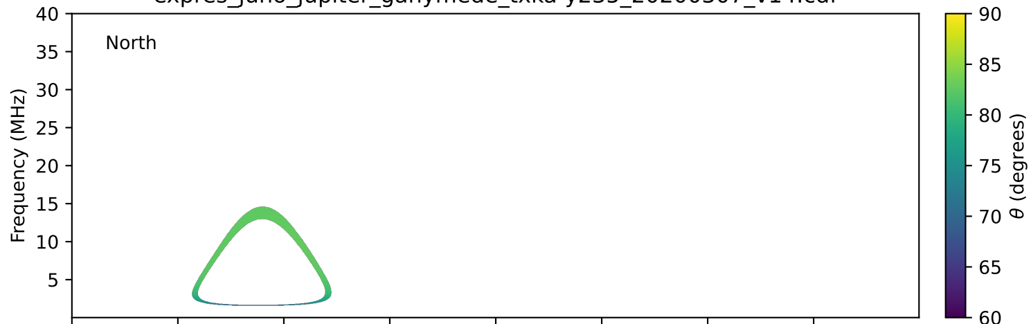
expres_juno_jupiter_ganymede_txka-y235_20200307_v14.cdf
