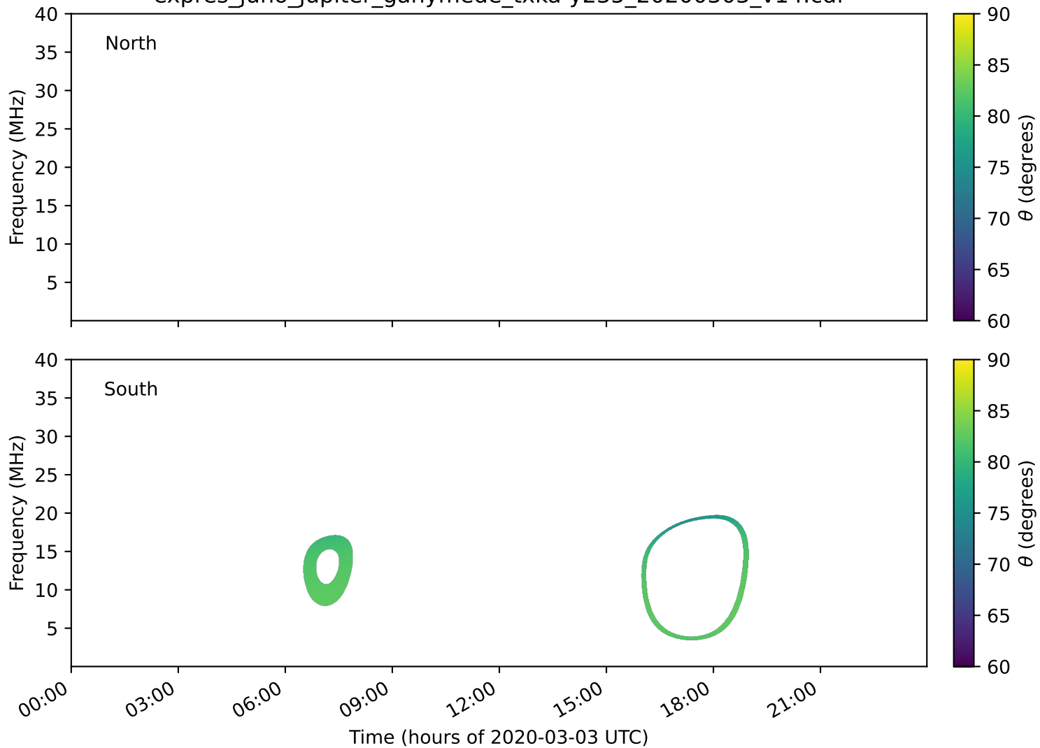
expres_juno_jupiter_ganymede_txka-y235_20200303_v14.cdf
