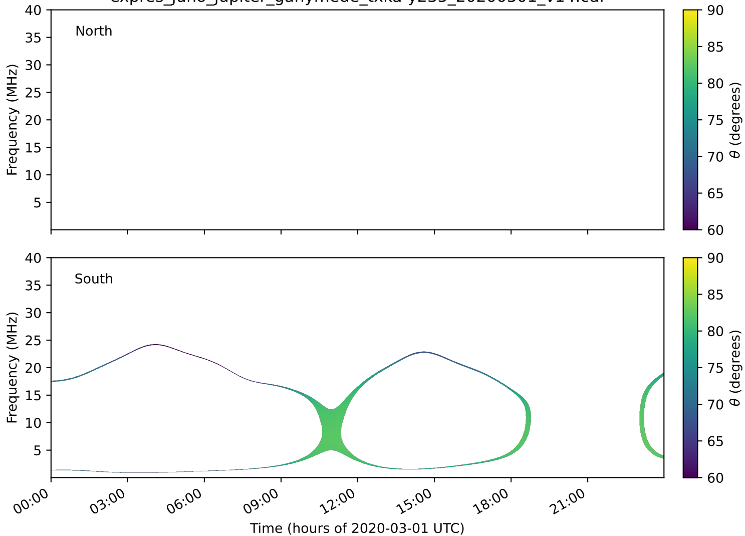
expres_juno_jupiter_ganymede_txka-y235_20200301_v14.cdf
