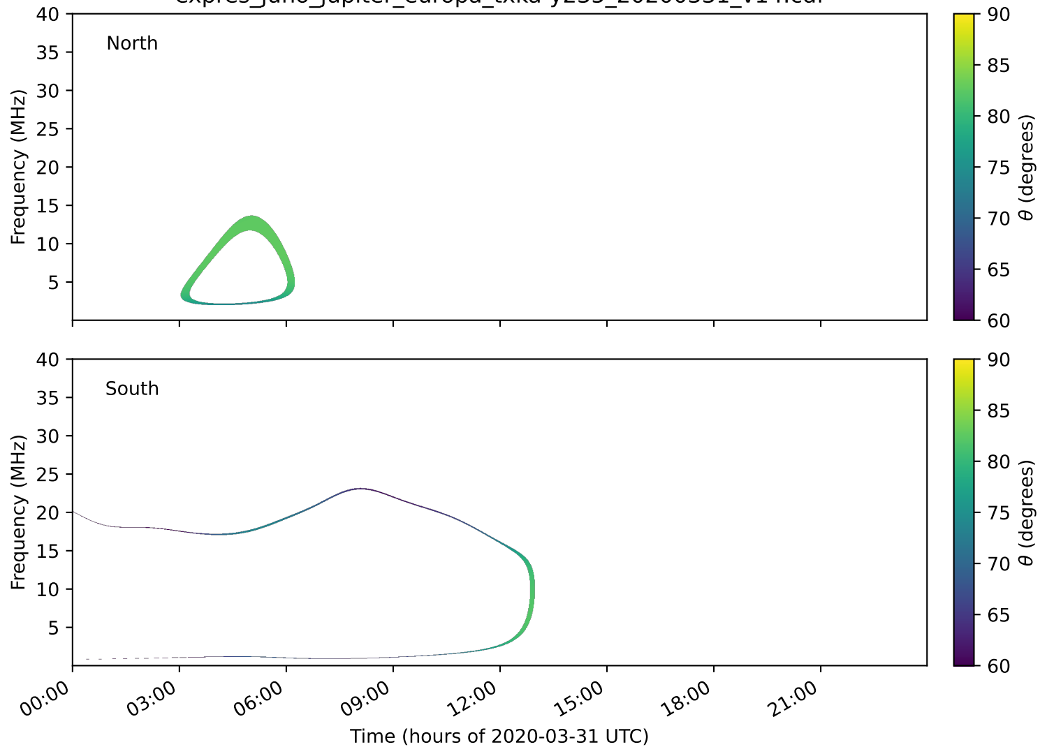
expres_juno_jupiter_europa_txka-y235_20200331_v14.cdf
