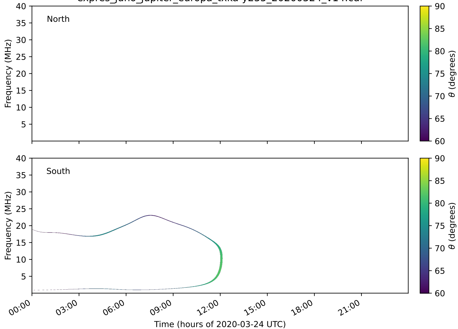
expres_juno_jupiter_europa_txka-y235_20200324_v14.cdf
