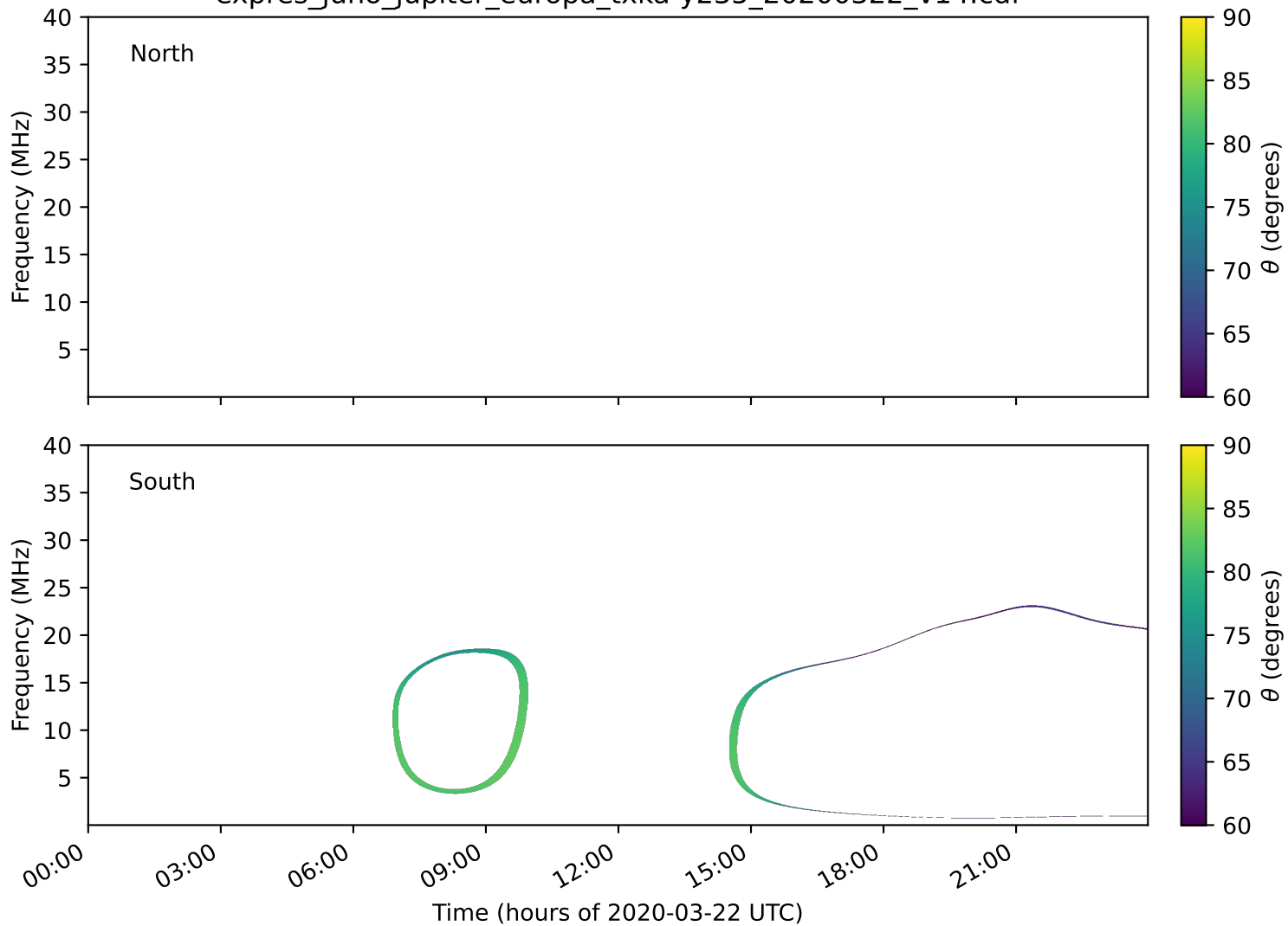
expres_juno_jupiter_europa_txka-y235_20200322_v14.cdf
