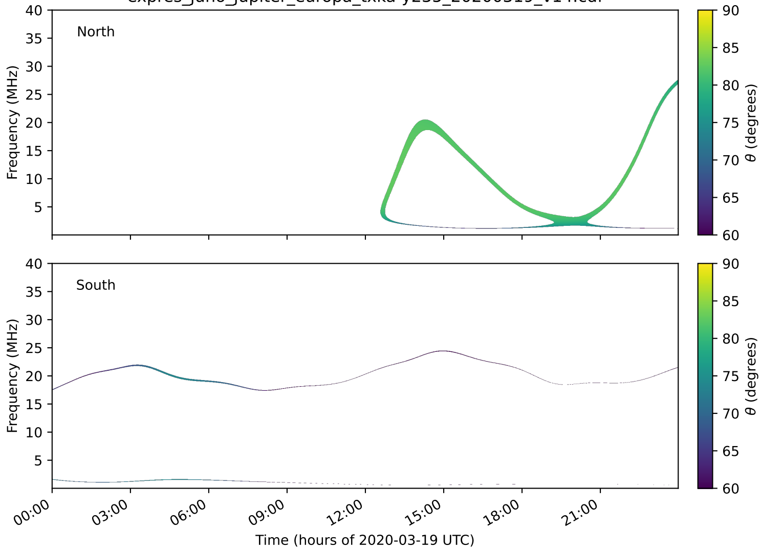
expres_juno_jupiter_europa_txka-y235_20200319_v14.cdf
