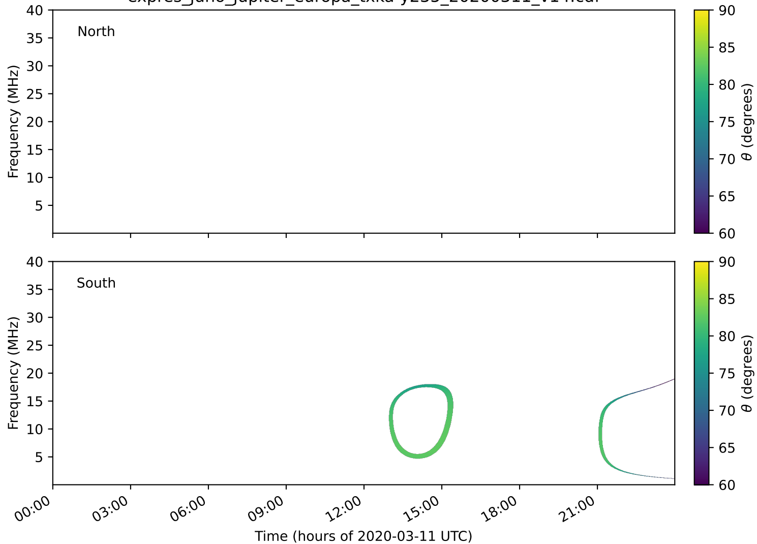
expres_juno_jupiter_europa_txka-y235_20200311_v14.cdf
