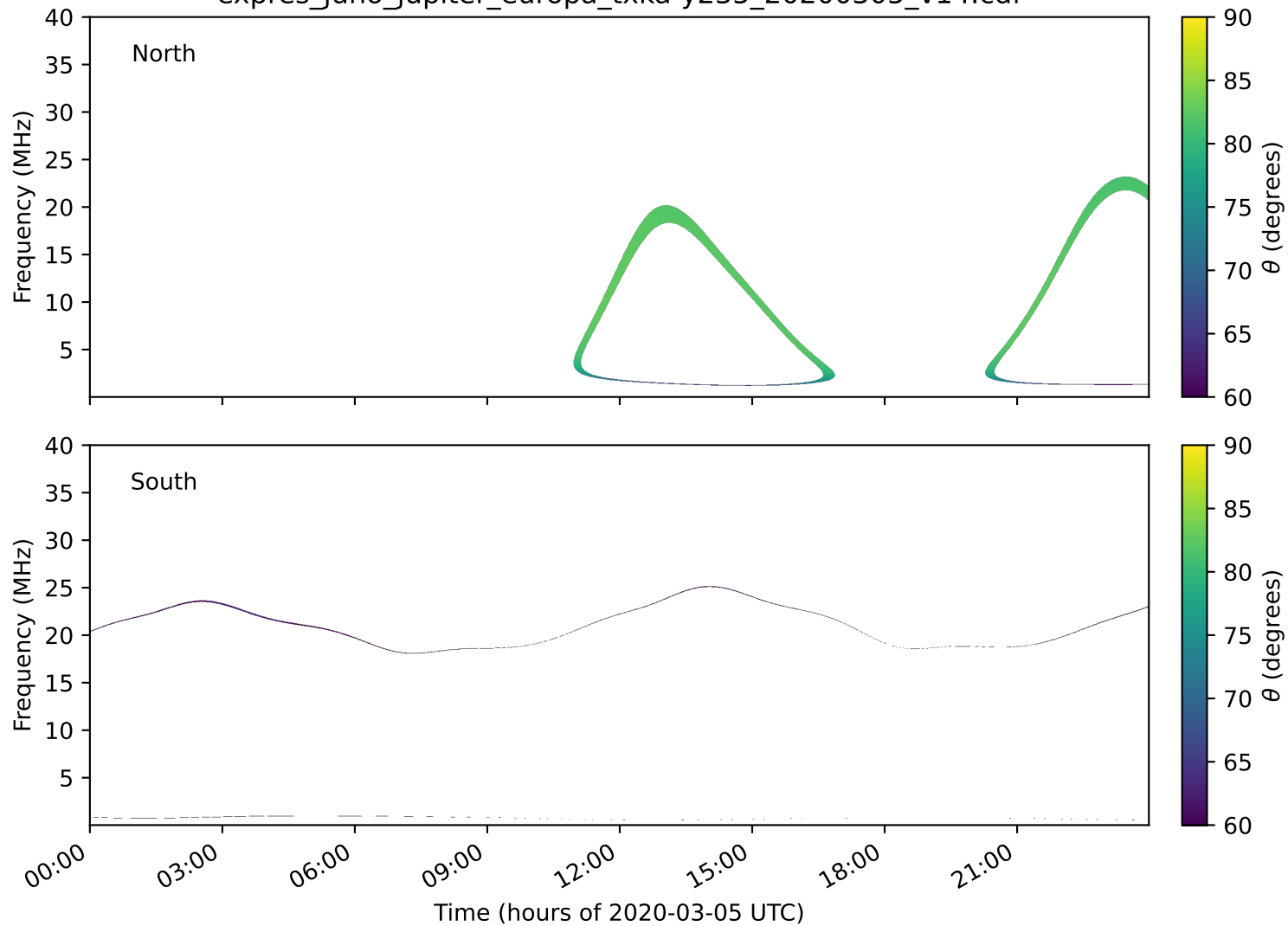
expres_juno_jupiter_europa_txka-y235_20200305_v14.cdf
