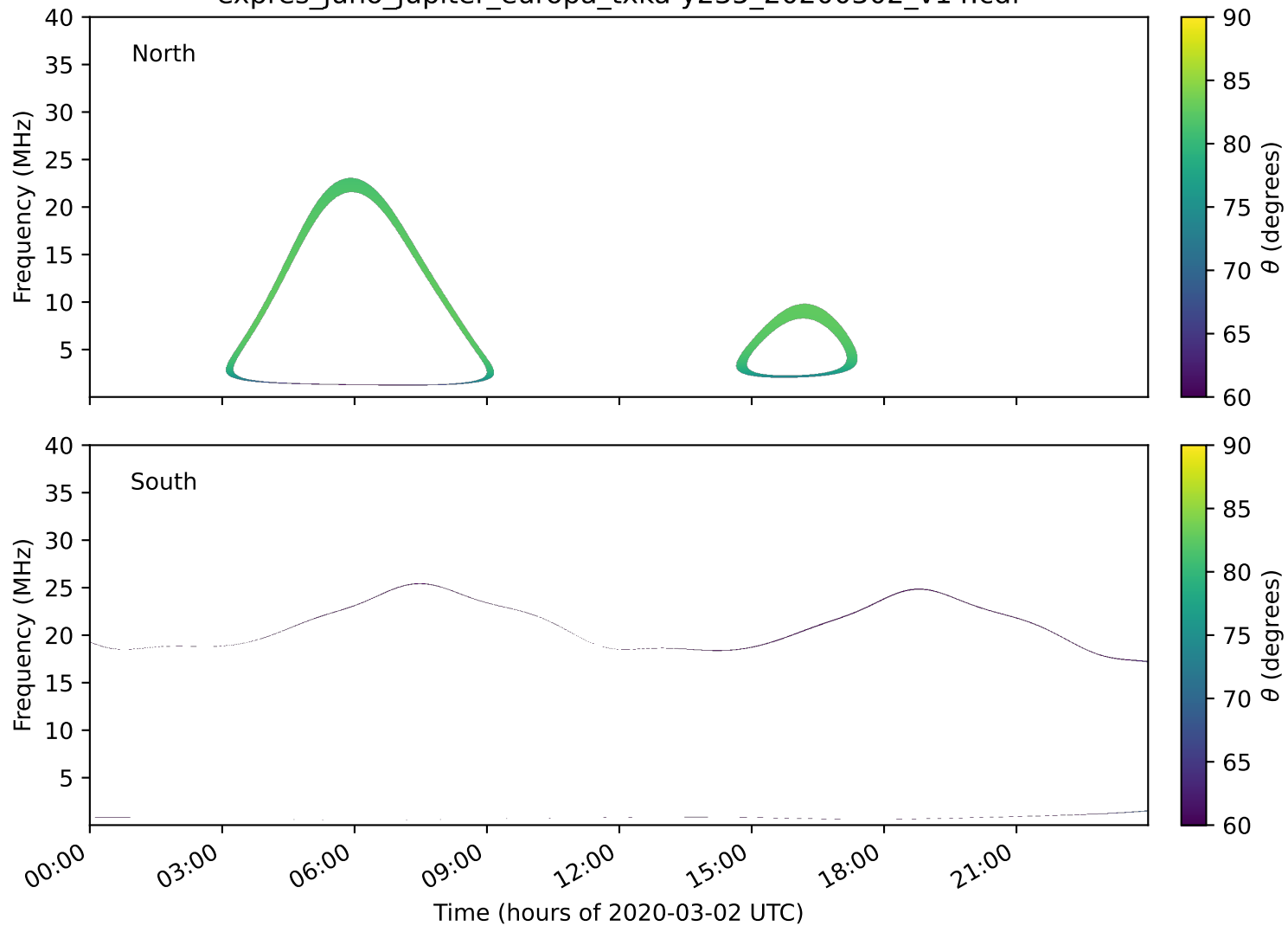
expres_juno_jupiter_europa_txka-y235_20200302_v14.cdf
