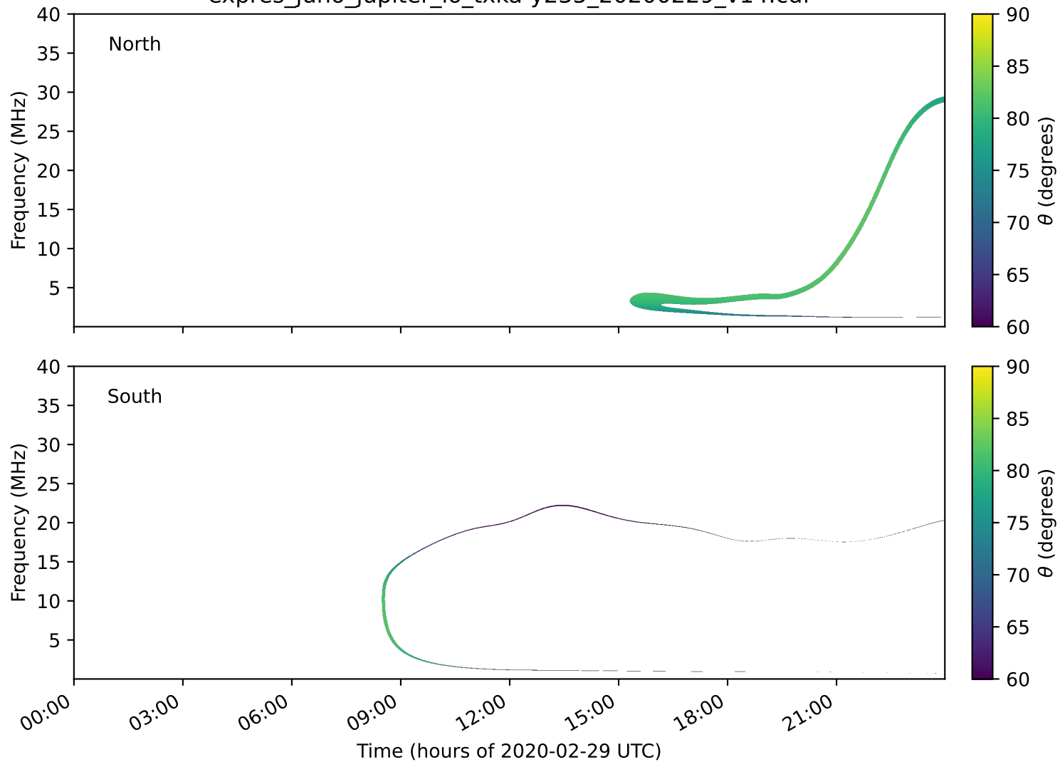
expres_juno_jupiter_io_txka-y235_20200229_v14.cdf
