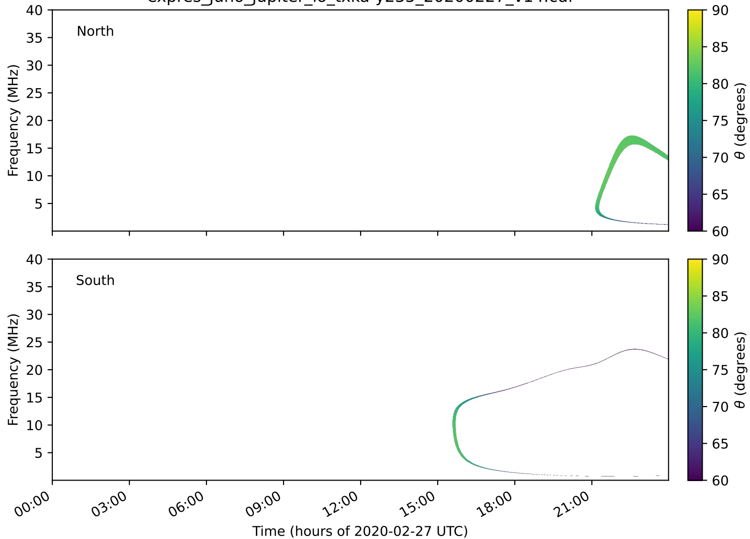
expres_juno_jupiter_io_txka-y235_20200227_v14.cdf
