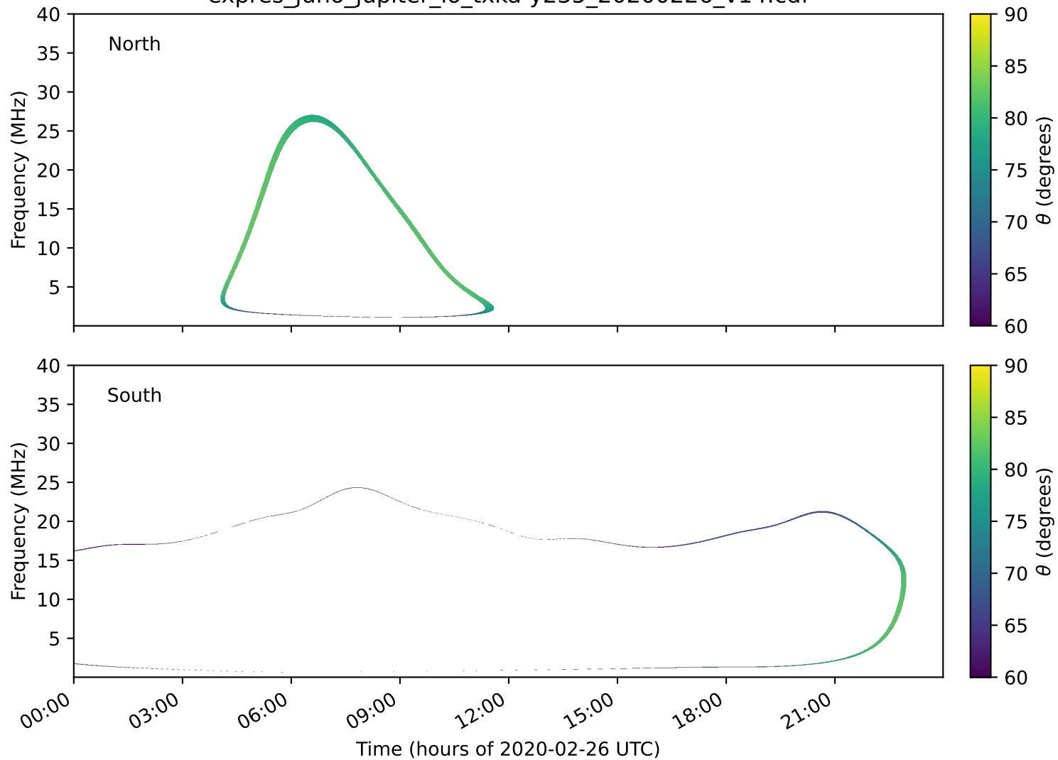
expres_juno_jupiter_io_txka-y235_20200226_v14.cdf
