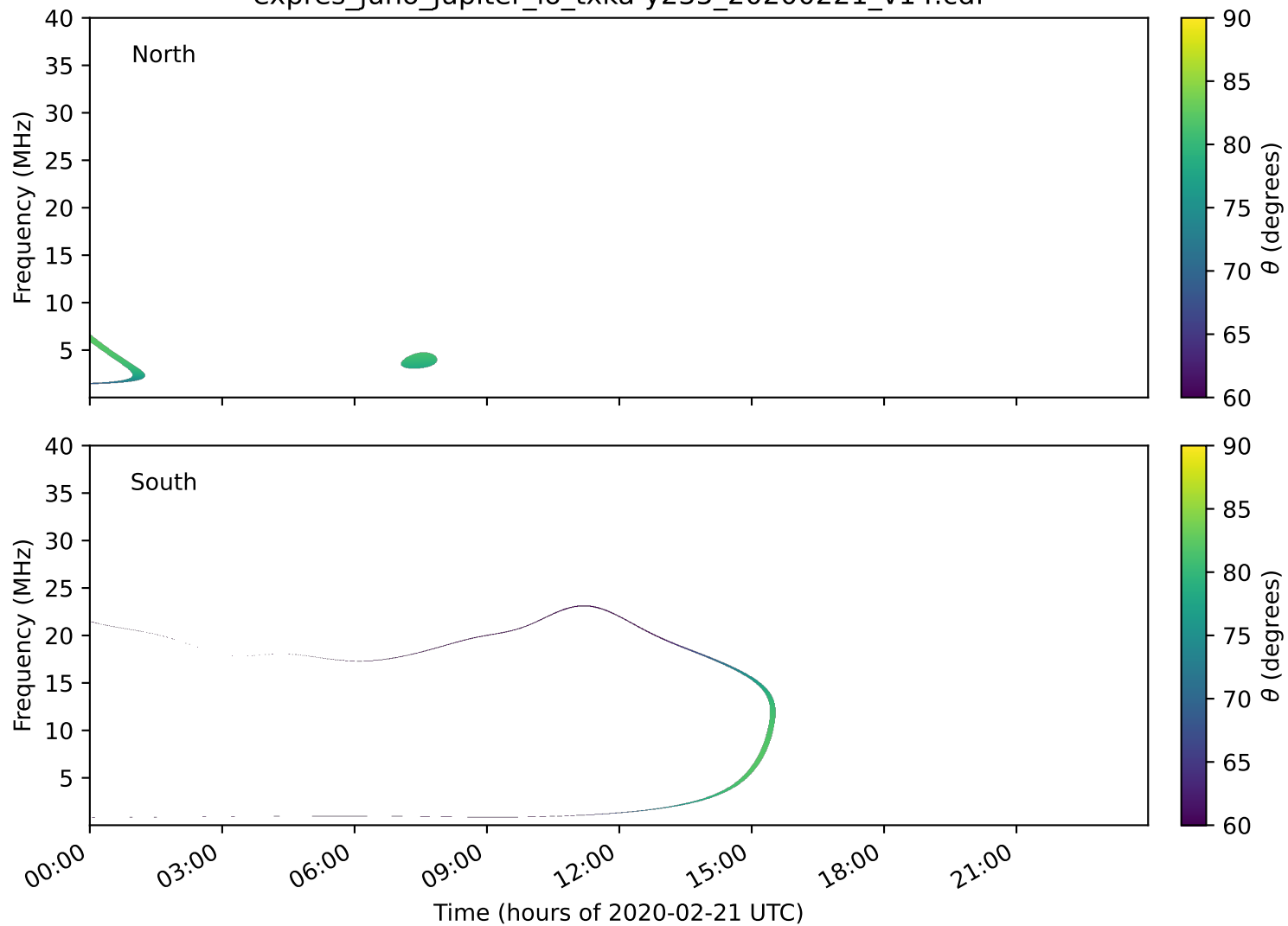
expres_juno_jupiter_io_txka-y235_20200221_v14.cdf
