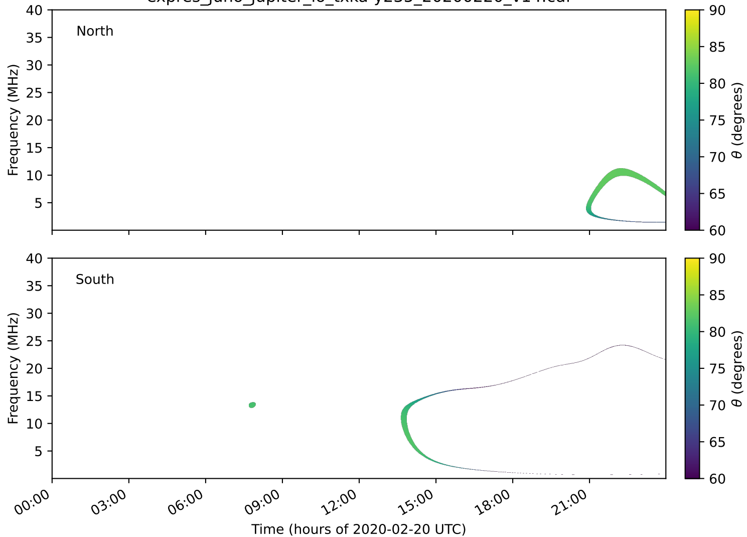
expres_juno_jupiter_io_txka-y235_20200220_v14.cdf
