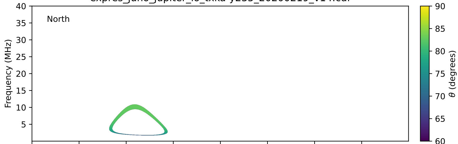
expres_juno_jupiter_io_txka-y235_20200219_v14.cdf
