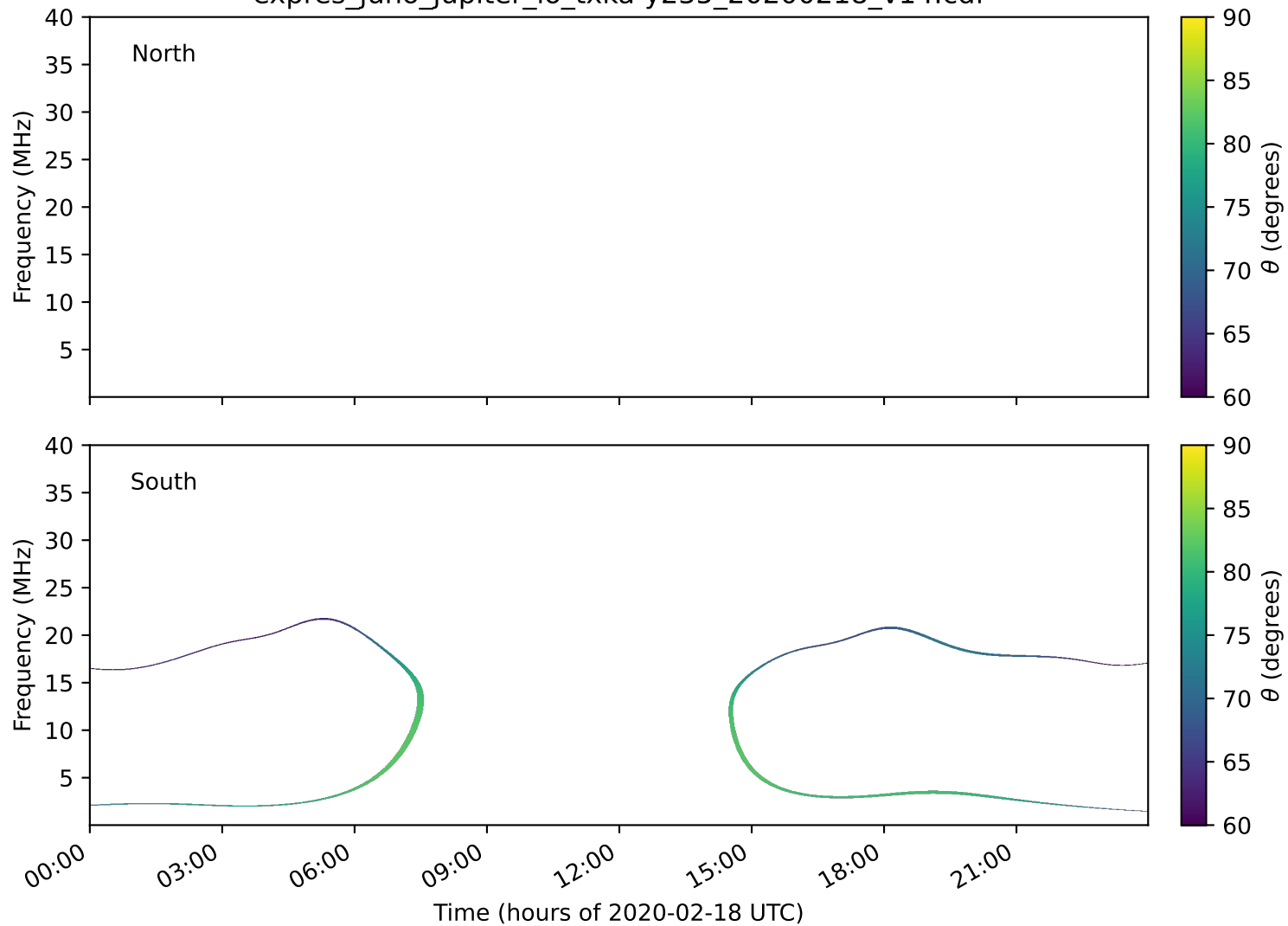
expres_juno_jupiter_io_txka-y235_20200218_v14.cdf
