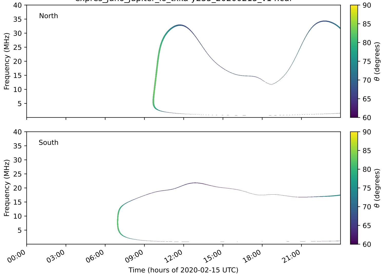
expres_juno_jupiter_io_txka-y235_20200215_v14.cdf
