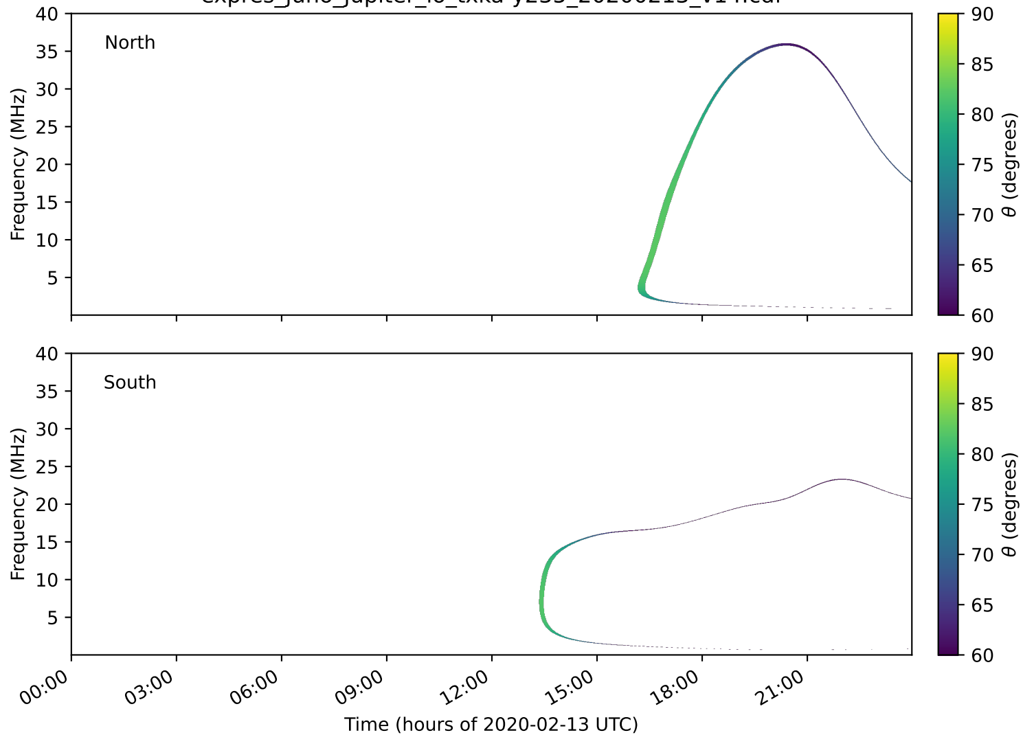
expres_juno_jupiter_io_txka-y235_20200213_v14.cdf
