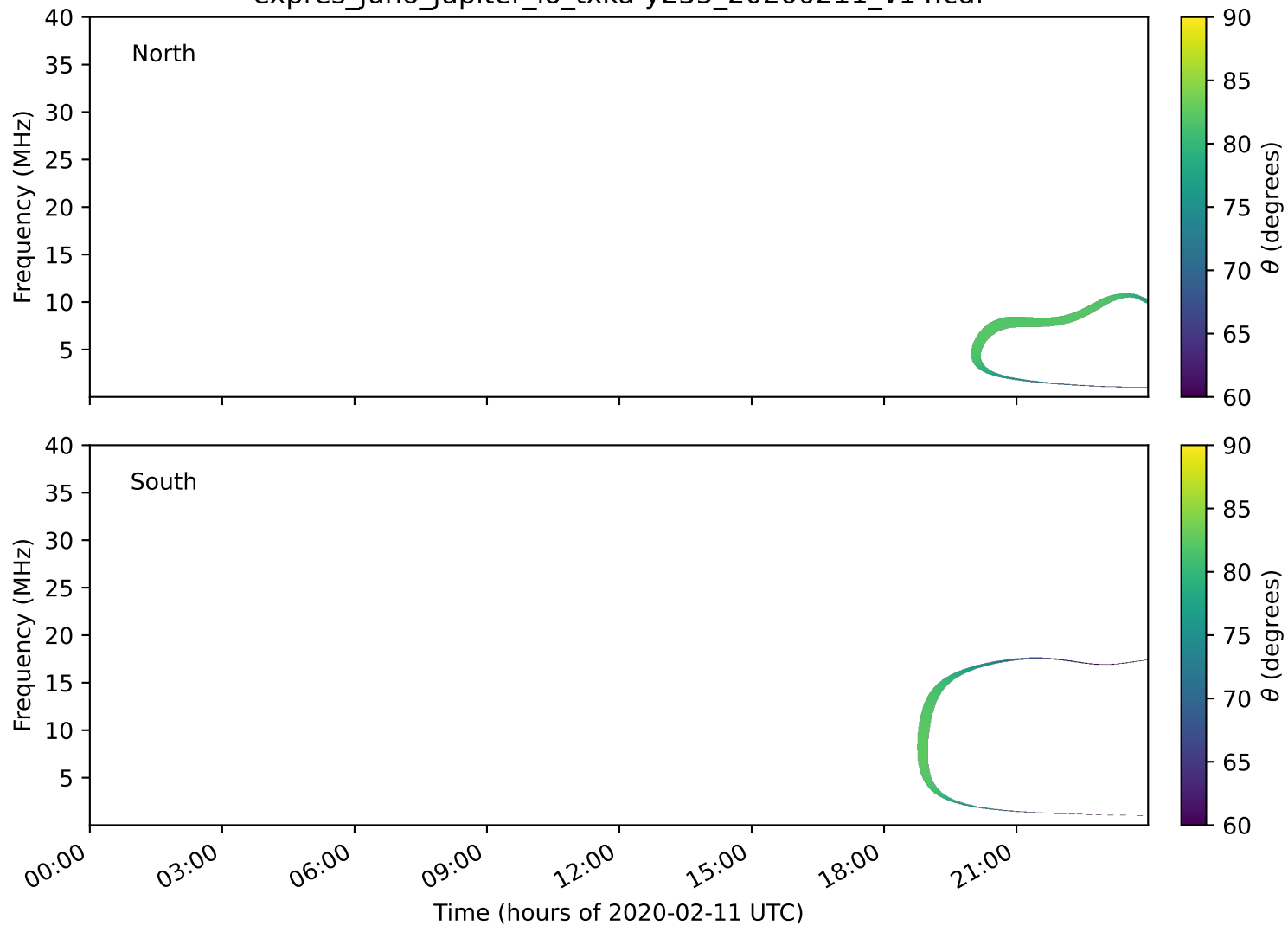
expres_juno_jupiter_io_txka-y235_20200211_v14.cdf
